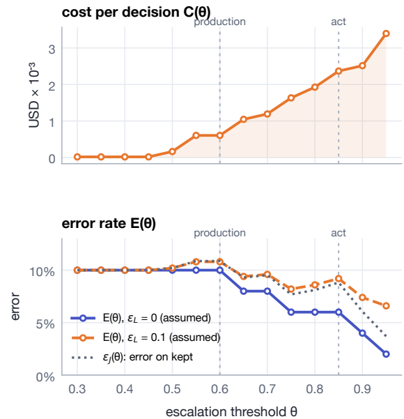
Figure 5: Error drops below Jev’s own 10.0% only where escalations make up almost all of the cost per decision, and how far it drops depends on an \varepsilon_L we did not measure. C(\theta) and E(\theta) on the 50 gold pairs. \varepsilon_L is assumed, not measured; the 29 escalation labels were too few for a curve.
