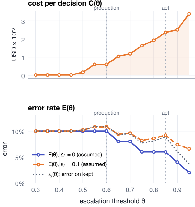
Figure 10: C(\theta) and E(\theta) on the 50 gold pairs. \epsilon_L is assumed, not measured; the 29 escalation labels were too few for a curve.
