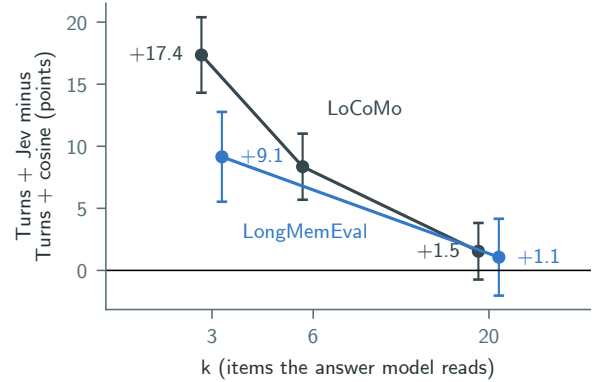
Figure 5: The rerank’s gain over similarity search (Turns + Jev minus Turns + cosine, paired, in points, with 95% intervals) against k . LoCoMo: 778 questions of the five held-out conversations at k=3 , k=6 and k=20 ; LongMemEval: 470 non-abstention questions, user and assistant turns, at k=3 and k=20 . The k=3 points are registered tests (S1, S7); the others are descriptive.
