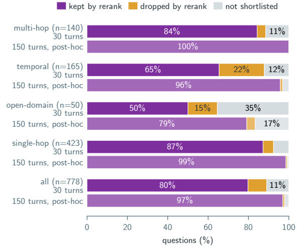
Figure 7: Where Turns + Jev’s accuracy stops, by category, on the 778 questions of the five held-out conversations: the rerank kept at least one evidence turn (purple), evidence was in the shortlist but the rerank kept none of it (amber), or no evidence turn was in the shortlist (grey). Upper bar of each pair: Turns + Jev’s 30-turn shortlist (shortlist recall, exploratory as registered). Lower, lighter bar: the wide variant’s 150-turn shortlist (post-hoc). Percentages are printed where the segment is wide enough.
