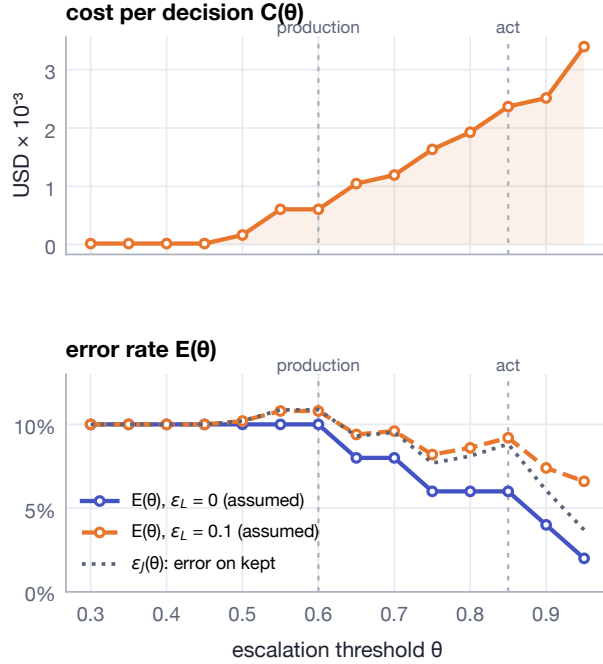
Figure 10: C(\theta) and E(\theta) on the 50 gold pairs. \varepsilon_L is assumed, not measured; the 29 escalation labels were too few for a curve.
