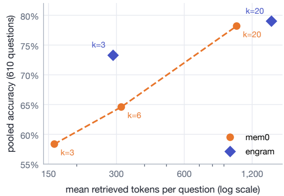
Figure 2: engram at k=3 sits above the line through mem0’s measured settings, and the two systems meet at k=20 : under a small budget, which memories are shown matters more than how many tokens. Pooled held-out accuracy (610 questions) against mean retrieved tokens per question. mem0 accuracy was measured at three settings, k=3, 6 and 20 ; the token-matching sweep counted tokens at the other k without answering. Models as in Table 2.
