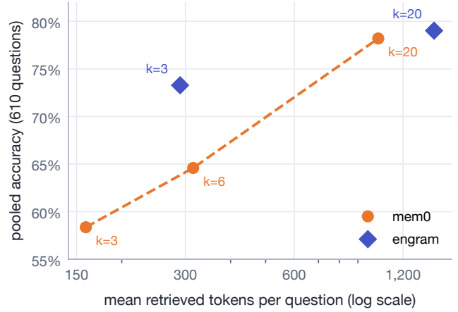
Figure 5: Pooled held-out accuracy (610 questions) against mean retrieved tokens per question. mem0 accuracy was measured at three settings, k=3, 6 and 20; the token-matching sweep counted tokens at the other k without answering. Models as in Table 3.
