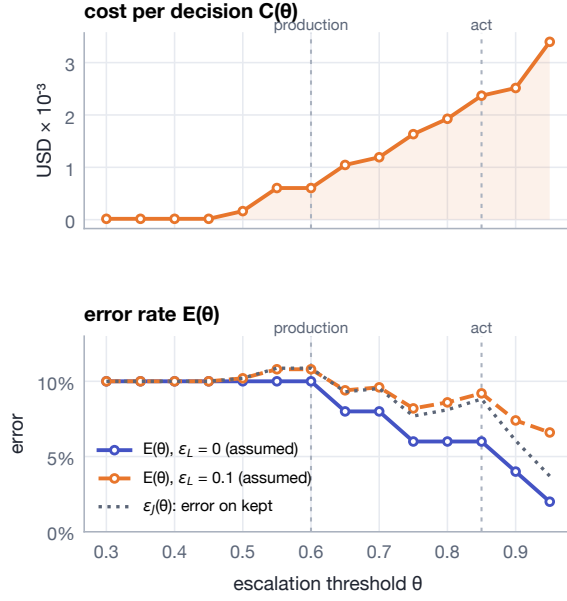
Figure 5: C(\theta) and E(\theta) on the 50 gold pairs. \varepsilon_L is assumed, not measured; the 29 escalation labels were too few for a curve. Error drops below Jev’s own 10.0% only where escalations make up almost all of the cost per decision, and how far it drops depends on an \varepsilon_L we did not measure.
