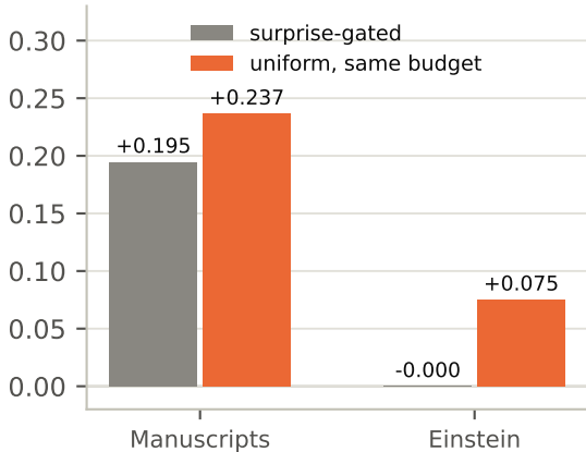
surprise gating hurts fast weights
