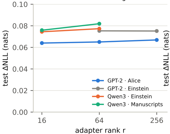
rank 16 is enough
