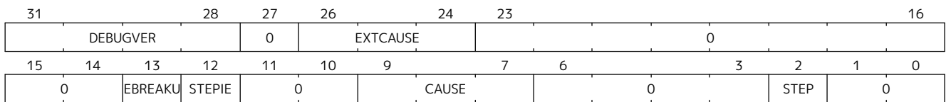
Register 3: U-mode or VU-mode debug control and status register ( udcsr )
