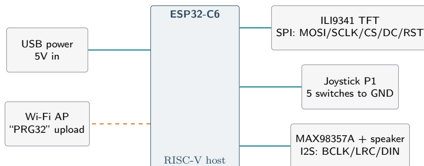
Figure E.1. The reference PRG32 board: a RISC-V ESP32-C6 with a display, a joystick, and an audio amplifier on its GPIO pins, powered over USB and exposing a Wi-Fi access point for cartridge upload (Montella et al., 2026c,g).
