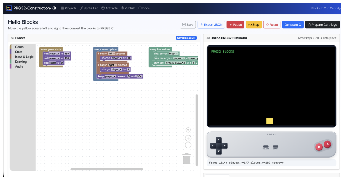
Figure 12.1. The Construction Kit. On the left are the blocks. On the right is the game screen, with a game pad under it (PRG32 Project, 2026a).
