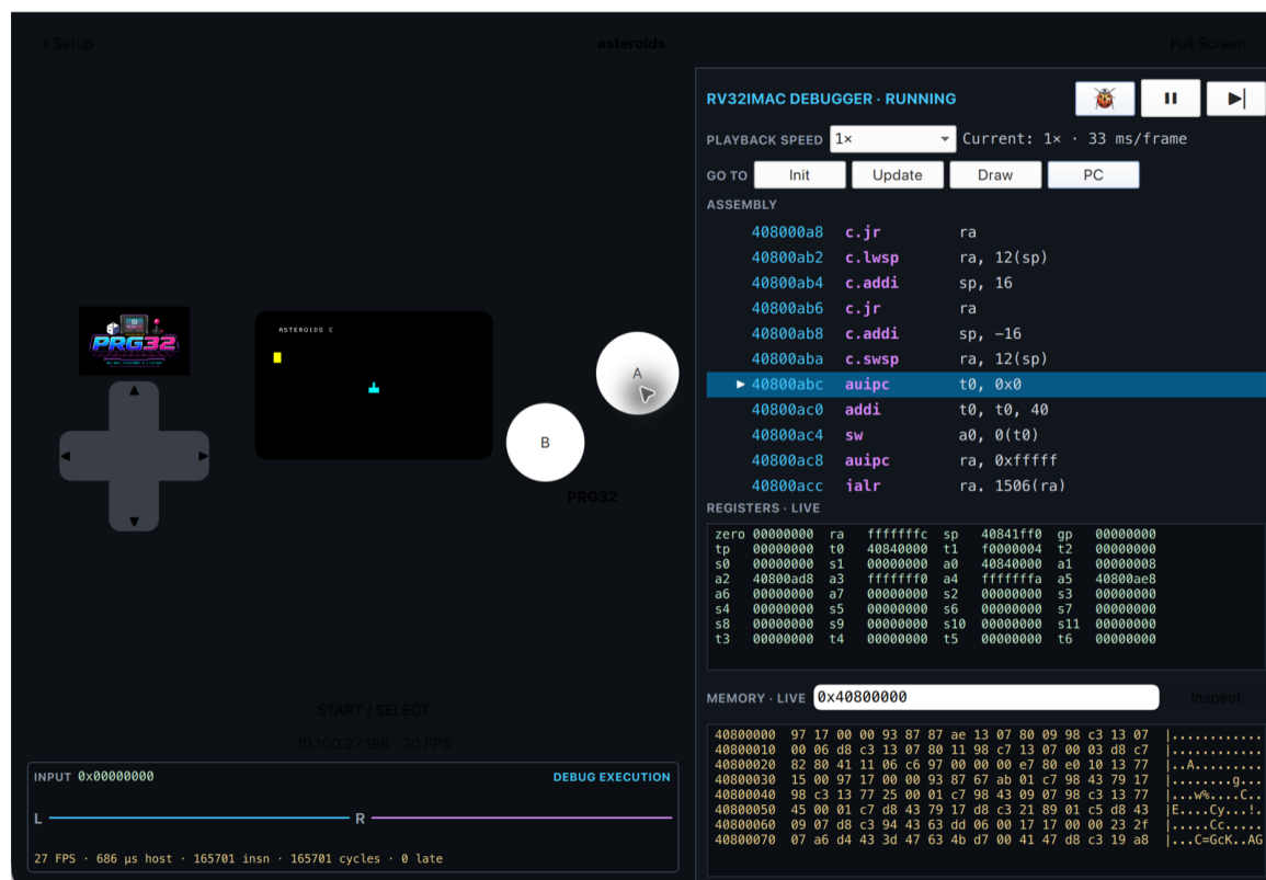
Figure 4.2. The PRG32-QT debugger: the running game, the live assembly listing with the next instruction highlighted, the registers, and a memory dump (Montella, 2026).
