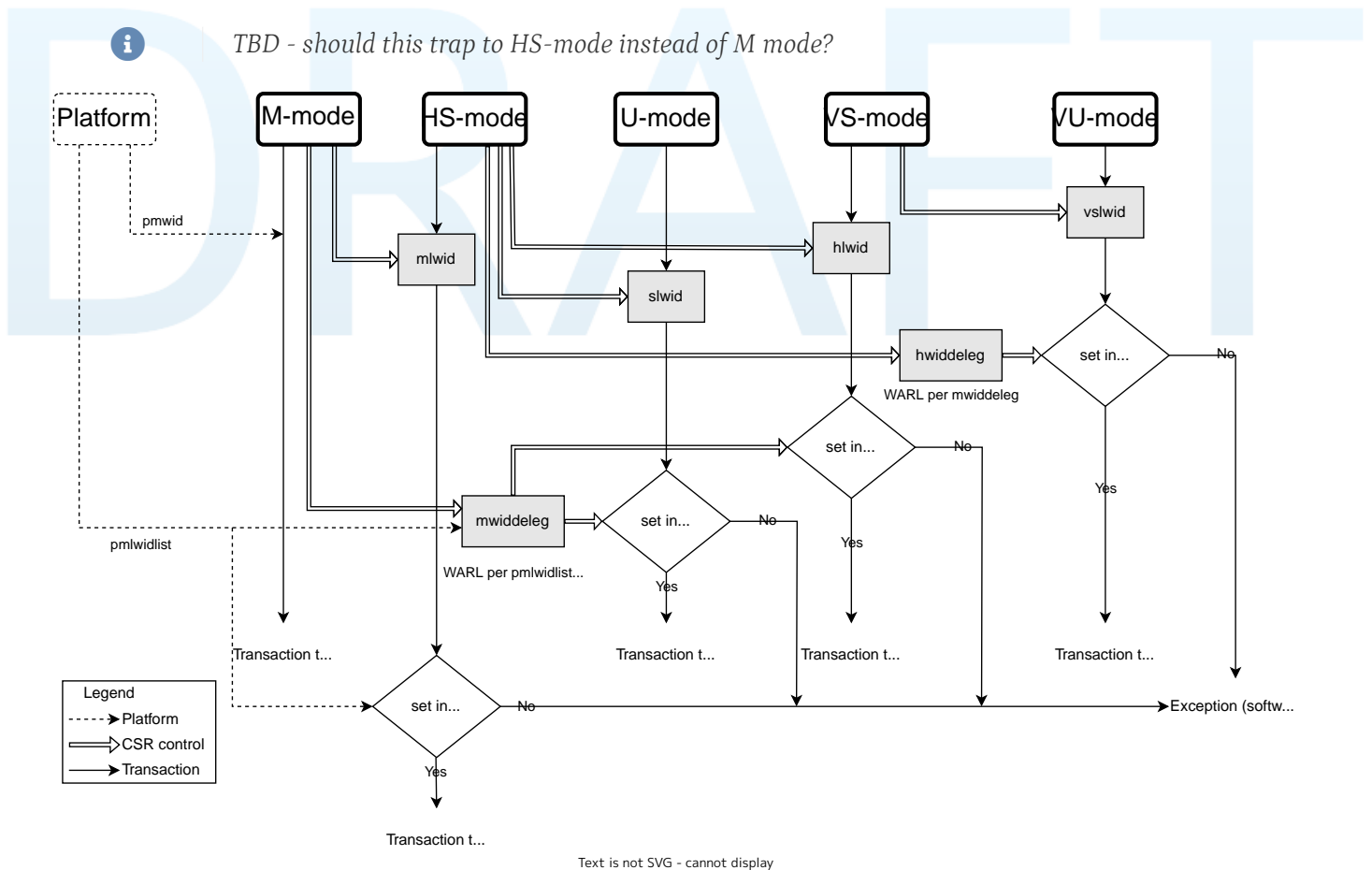
Figure 130. Shwdeleg/Svswid extensions: Support for HS-mode to control the lower privilege mode's world.
