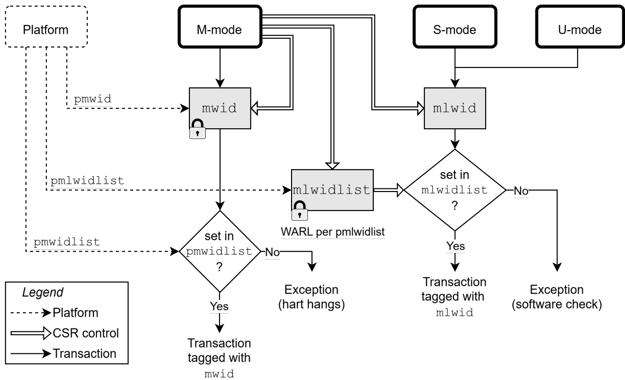
Figure 128. Smlwidlist extension, shown here with the Smwid and Smlwid dependencies.
