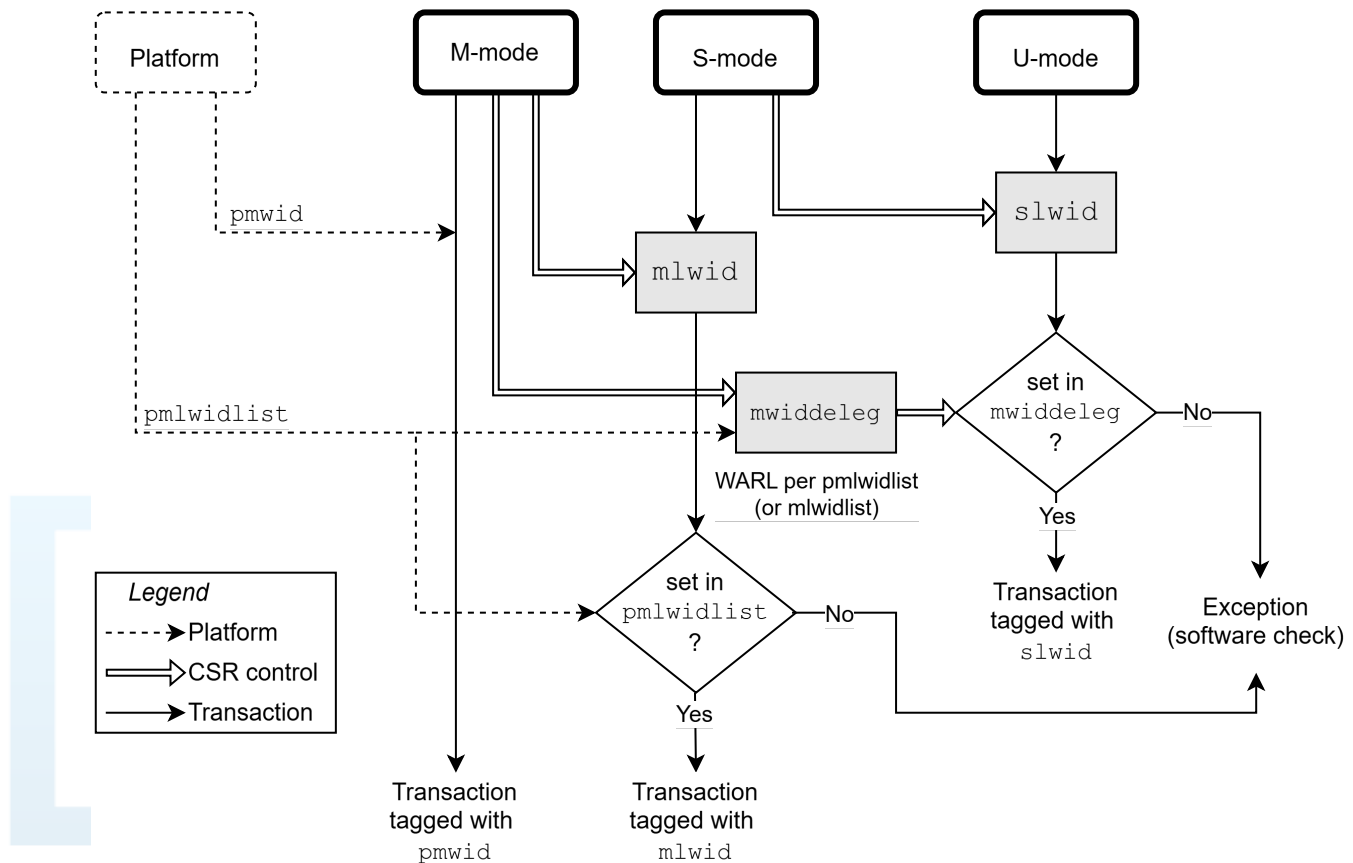
Figure 129. Smwdeleg/Sswid extensions: Support for S-mode to control U-mode's world. Shown here without Smwid or Smlwidlist.
