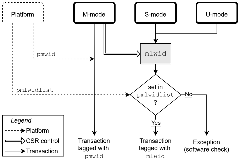
Figure 127. Smlwid extension: Support for M-mode to control lower privilege modes' world, shown here without Smwid.
