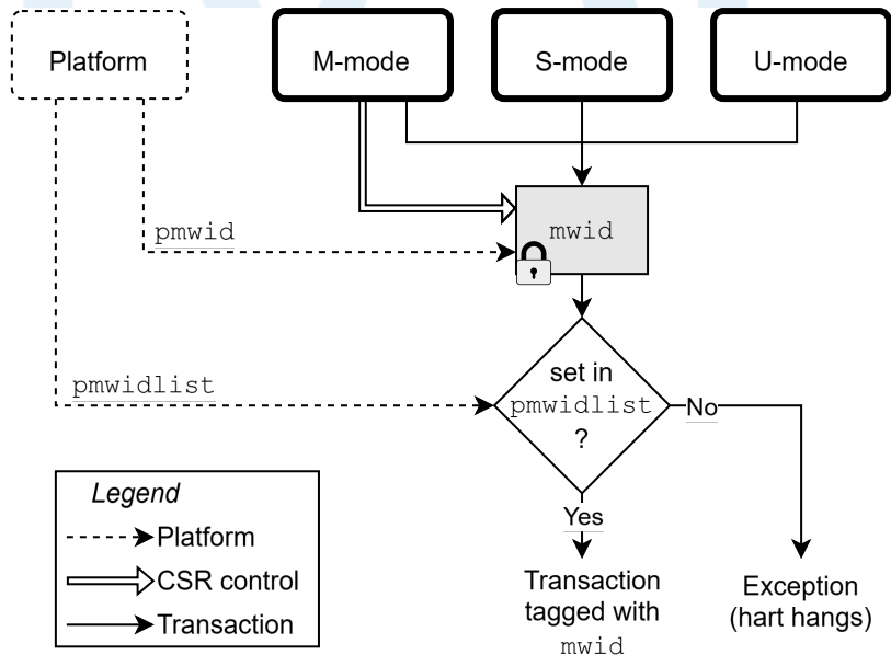
Figure 126. One world with the Smwid extension
