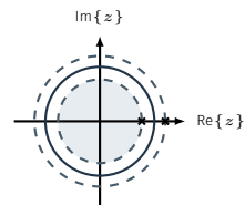
|z| < 0.8 : anti-causal, unstable
