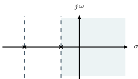
\operatorname{Re}\{s\} > -1 : causal, stable
