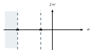
\operatorname{Re}\{s\} < -3 : anti-causal, unstable
