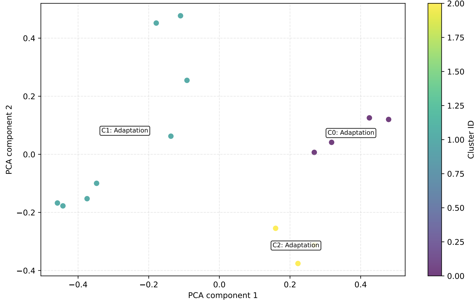
RQ2: MiniLM Embedding-Based Clustering Documents = 15, Clusters = 3, Silhouette = 0.187
