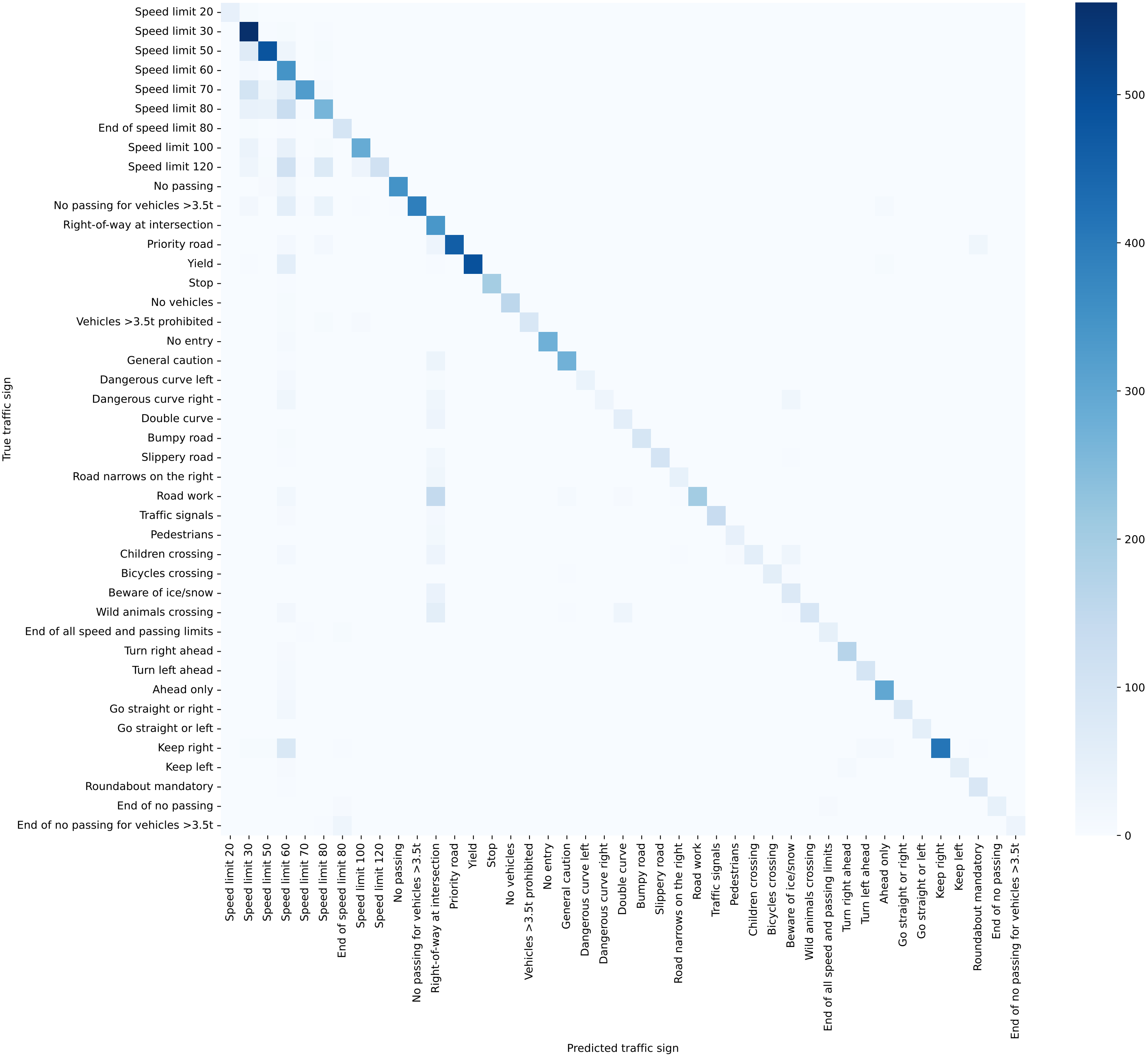
Confusion Matrix - GTSRB for ResNet50 Tranfer learning MODEL
