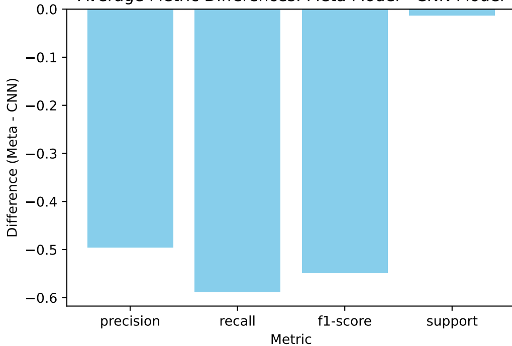
Average Metric Differences: Meta Model - CNN Model
