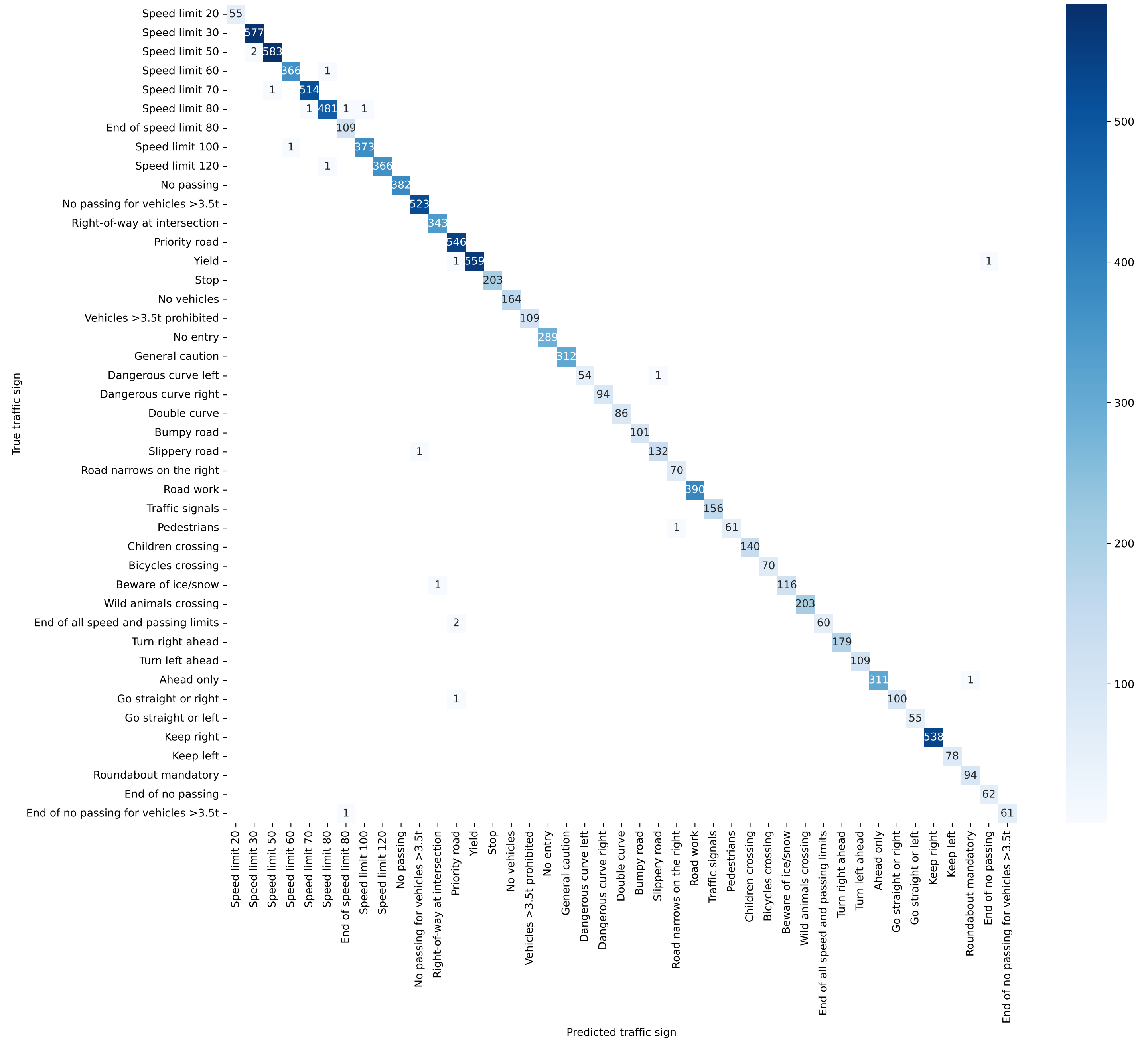
Confusion Matrix: GTSRB for Custom CNN Model
