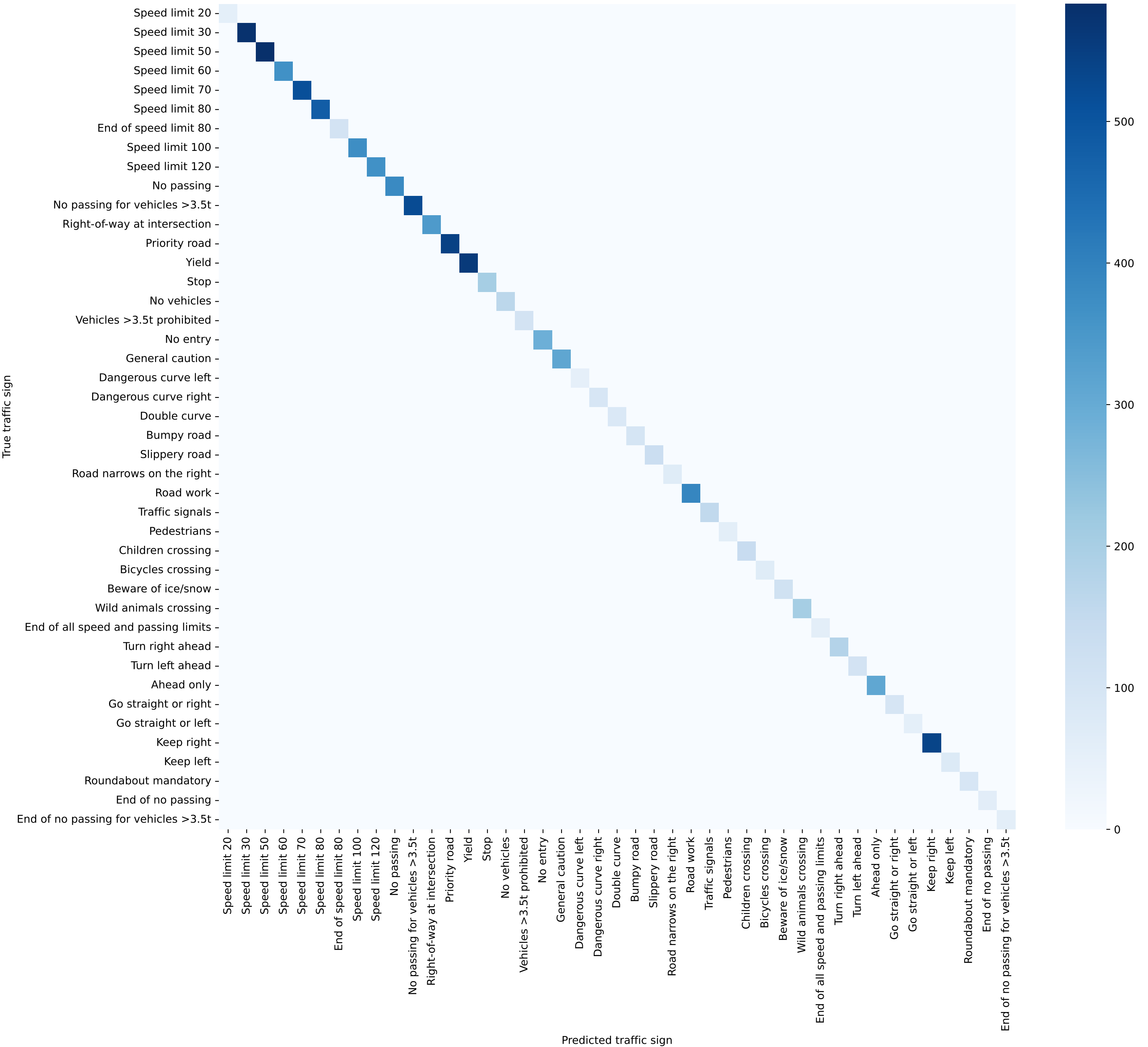
Confusion Matrix - GTSRB for Custom CNN Model
