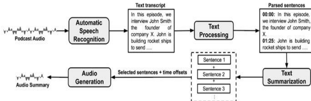
Figure 3.2 PodSumm Architecture
