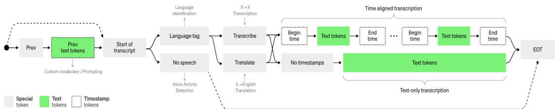
Figure 3.6 Phrase-level timestamps, multilingual speech transcription, and to-English speech translation
