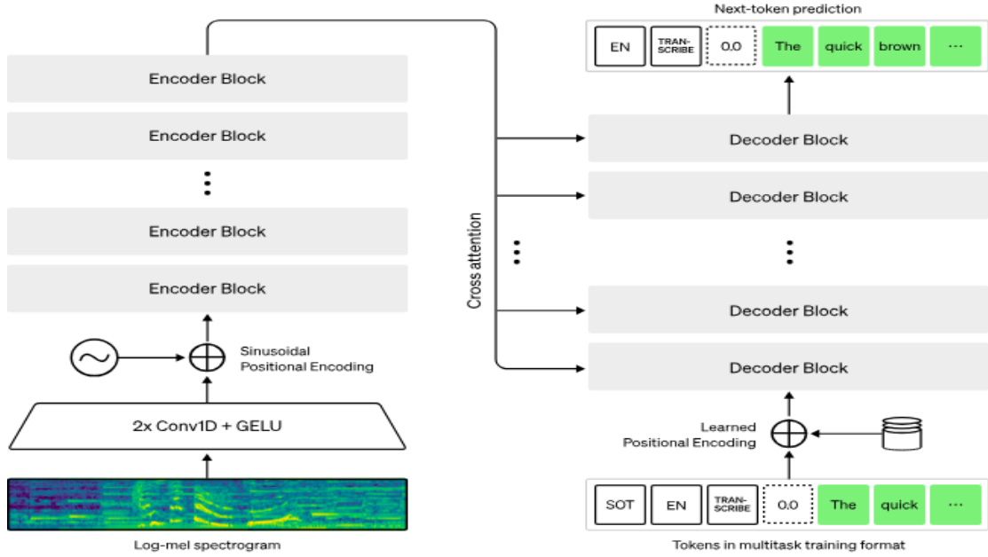
Figure 3.5 Whisper architecture
