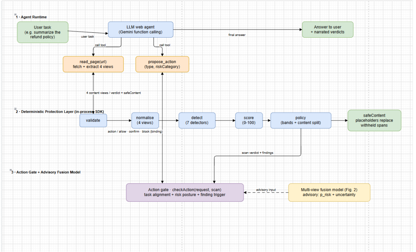
Fig. 1. Overall architecture of the proposed CtxVigil system: the LLM web agent’s tool calls are routed through the protection layer, whose scan pipeline, action gate, and advisory multi-view fusion model decide what the agent may read and do.
