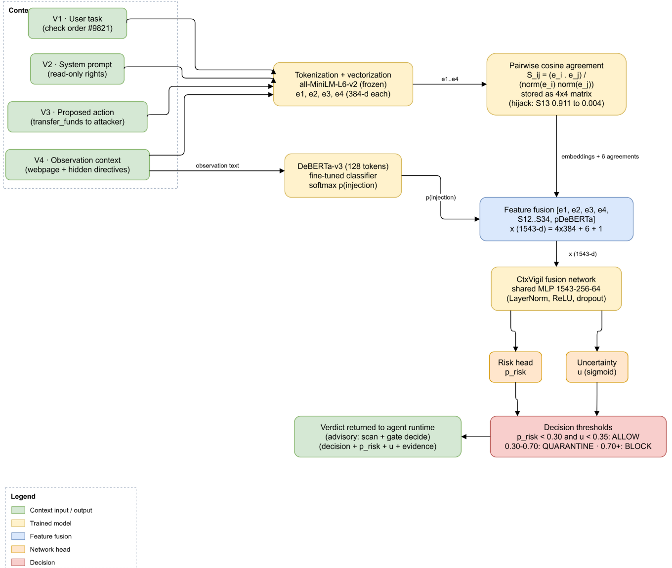
Fig. 2. Detailed data-flow of the protection layer. The agent runtime supplies four context views: user task, system prompt, proposed action, and observation. Tokenization and vectorization with the frozen all-MiniLM-L6-v2 encoder produce four 384-d embeddings, whose pairwise cosine similarities are stored in the 4×4 agreement matrix (in the InjecAgent hijack fixture the task-action agreement S13 collapses from 0.911 to 0.004). In parallel, the observation text passes through the fine-tuned DeBERTa-v3 classifier to yield p(\text{injection}) . The concatenated 1,543-d feature vector feeds the CtxVigil fusion network, whose risk and uncertainty heads drive the thresholded ALLOW / QUARANTINE / BLOCK decision that is returned to the agent runtime.
