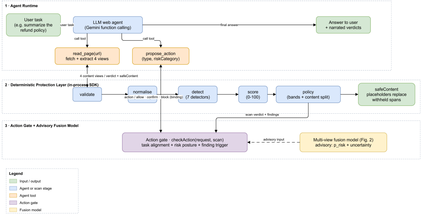
Fig. 1. End-to-end application flow. (1) The Gemini agent’s only two tools route through the protection layer: read_page fetches the page and receives only safeContent back, and propose_action receives the gate’s binding decision. (2) The deterministic layer validates, normalises the page into four content views, detects, scores, and partitions content. (3) The multi-view fusion model of Fig. 2 evaluates the episode and contributes an advisory verdict to the gate.
