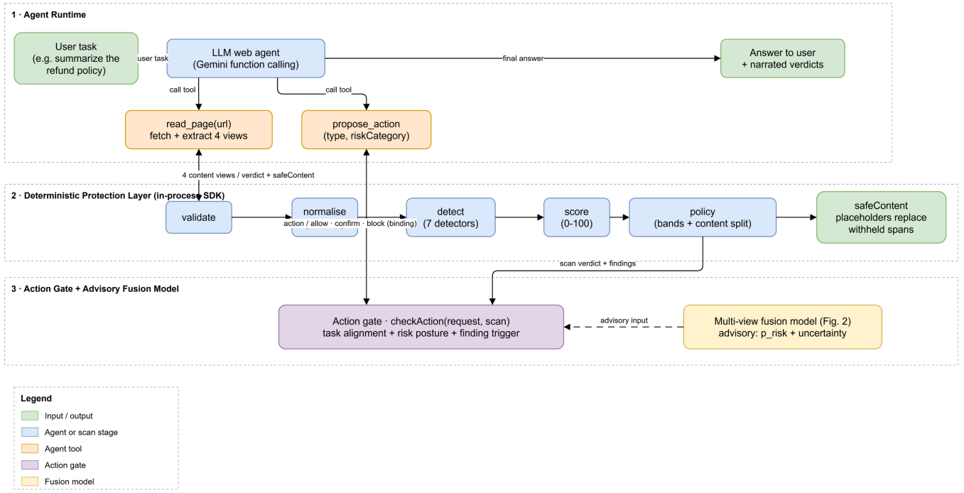
Fig. 1. End-to-end application flow. (1) The Gemini agent’s only two tools route through the protection layer: read_page fetches the page and receives only safeContent back, and propose_action receives the gate’s binding decision. (2) The deterministic layer validates, normalises the page into four content views, detects, scores, and partitions content. (3) The multi-view fusion model of Fig. 2 evaluates the episode and contributes an advisory verdict to the gate.
