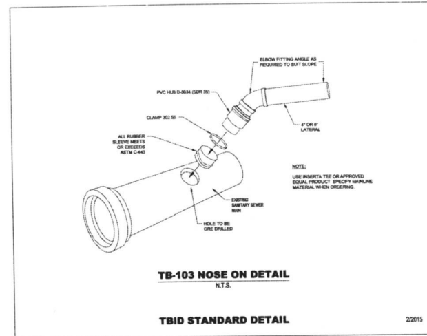
SEWER LATERAL CONNECTION ① SCALE: NTS
