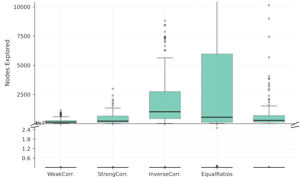
Branch & Bound Nodes Explored by Instance Family
