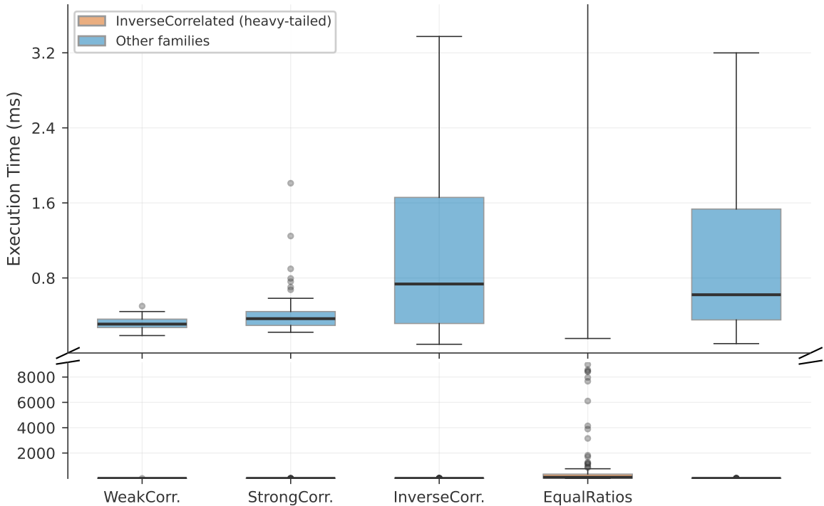
Branch & Bound Runtime at n=1000 by Instance Family
