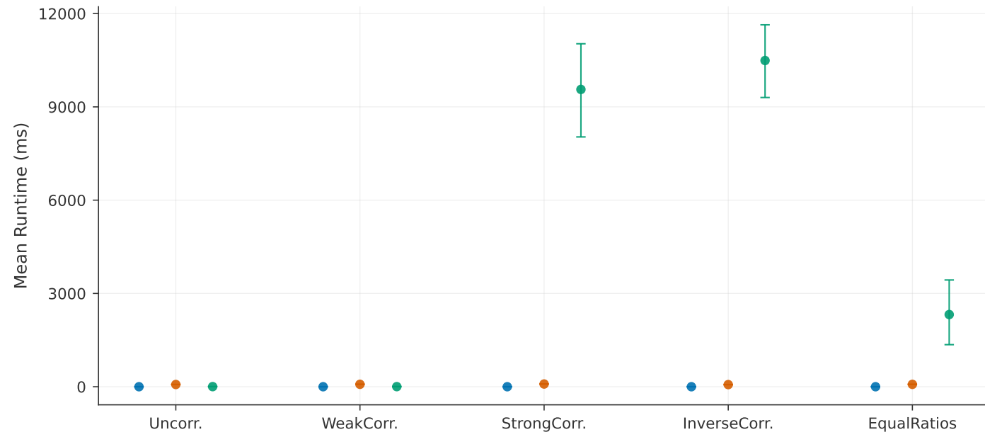
Execution Time at n=500 by Algorithm and Instance Family Execution Time at n=1000
