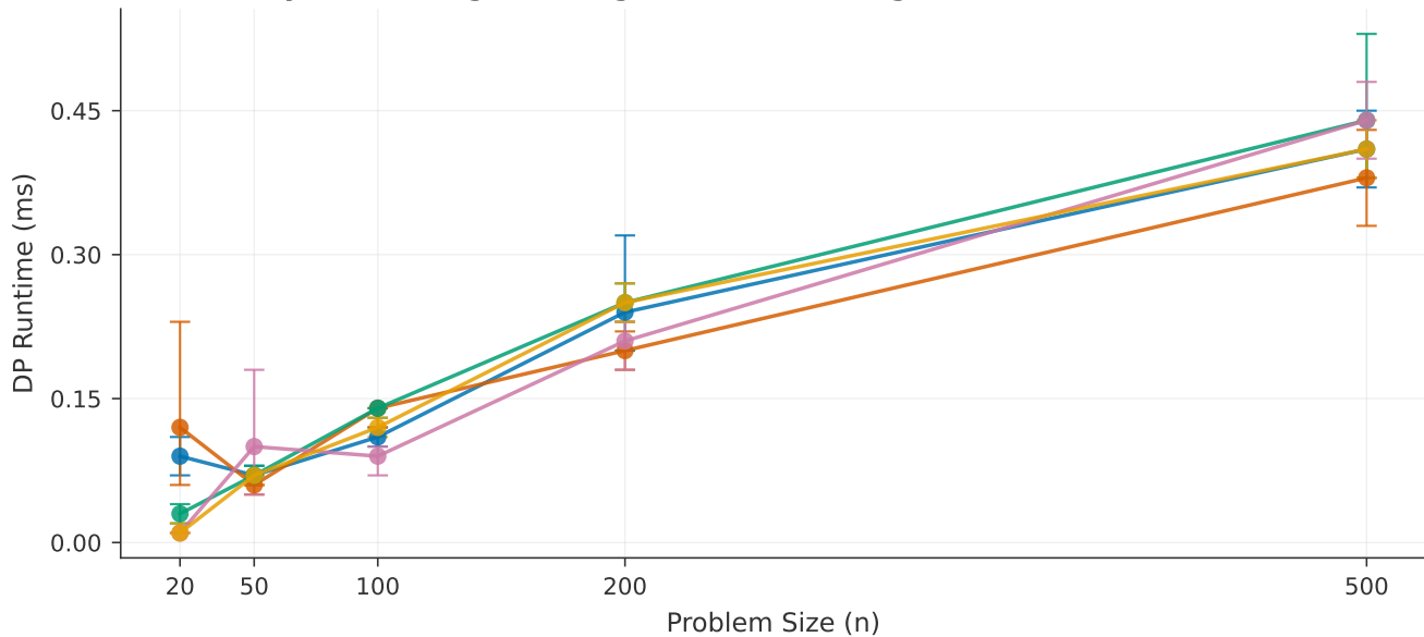
Dynamic Programming Runtime Scaling with n ( W=1000 fixed)
