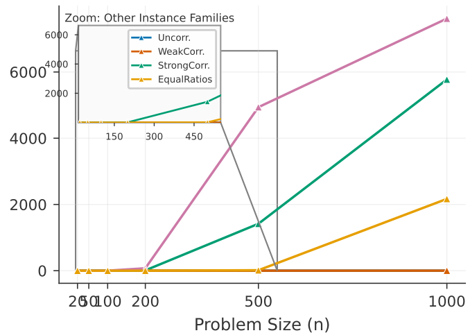
BranchAndBound
