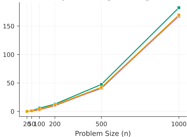
DynamicProgramming
