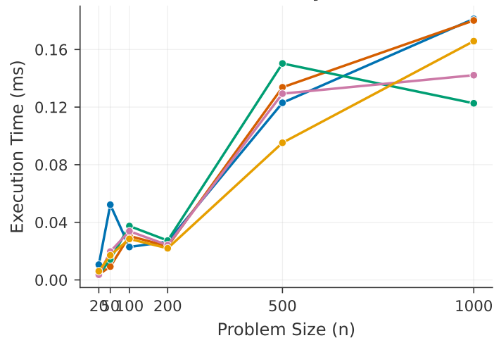
Greedy
