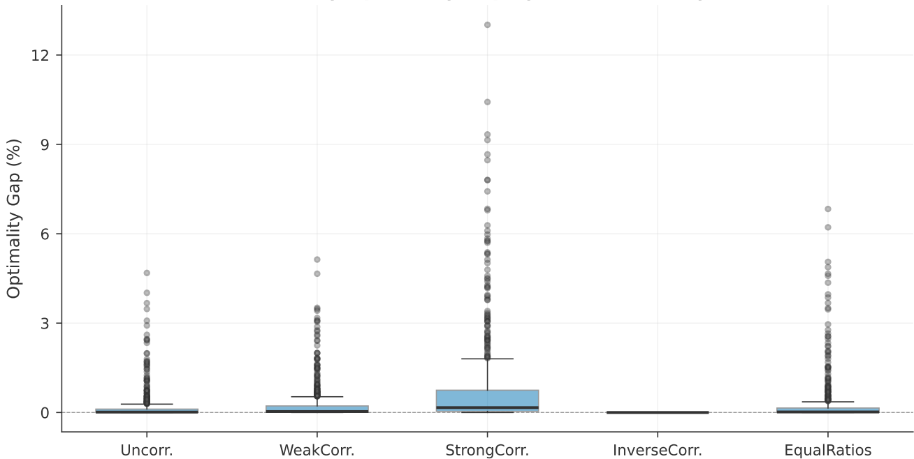
Greedy Optimality Gap by Instance Family
