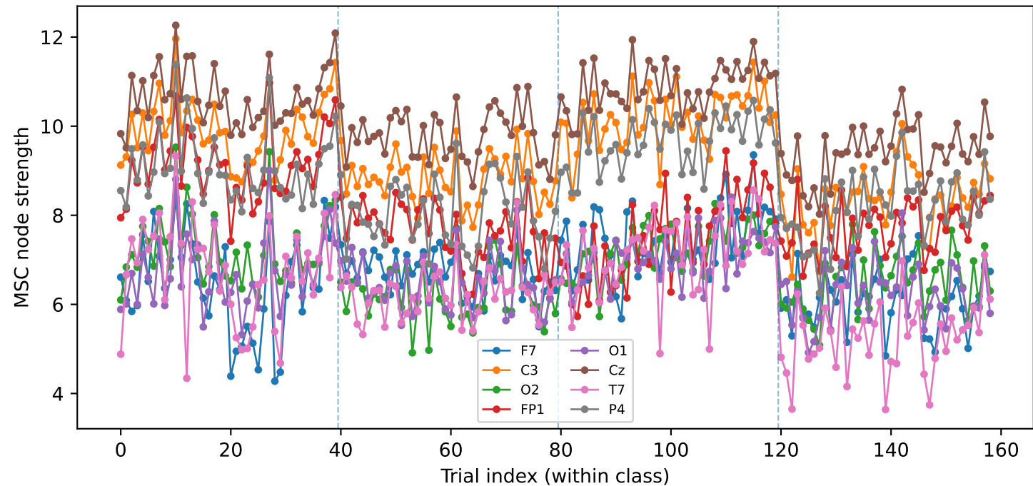
S21 MSC - NS trajectories (R)
