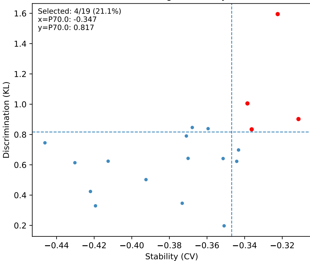
S09 wPLI - Node strength: stability (-CV) vs KL
