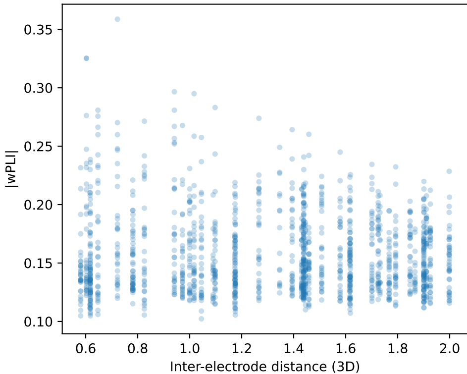
wPLI vs distance, class R
