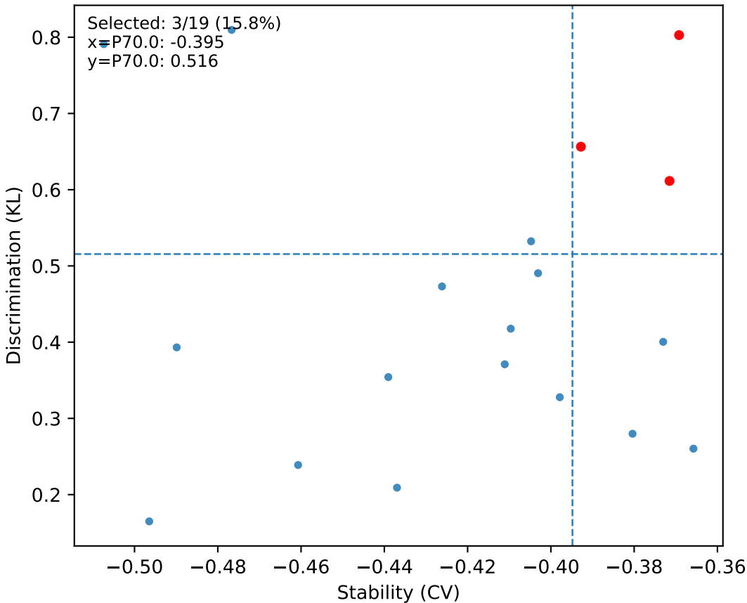
S21 wPLI - Node strength: stability (-CV) vs KL
