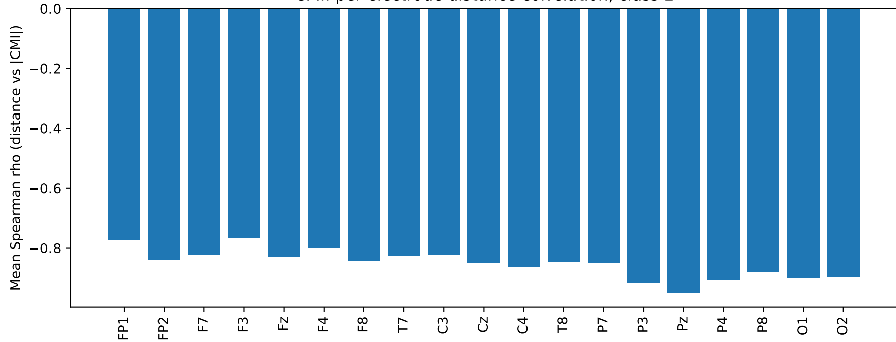
CMI: per-electrode distance correlation, class L
