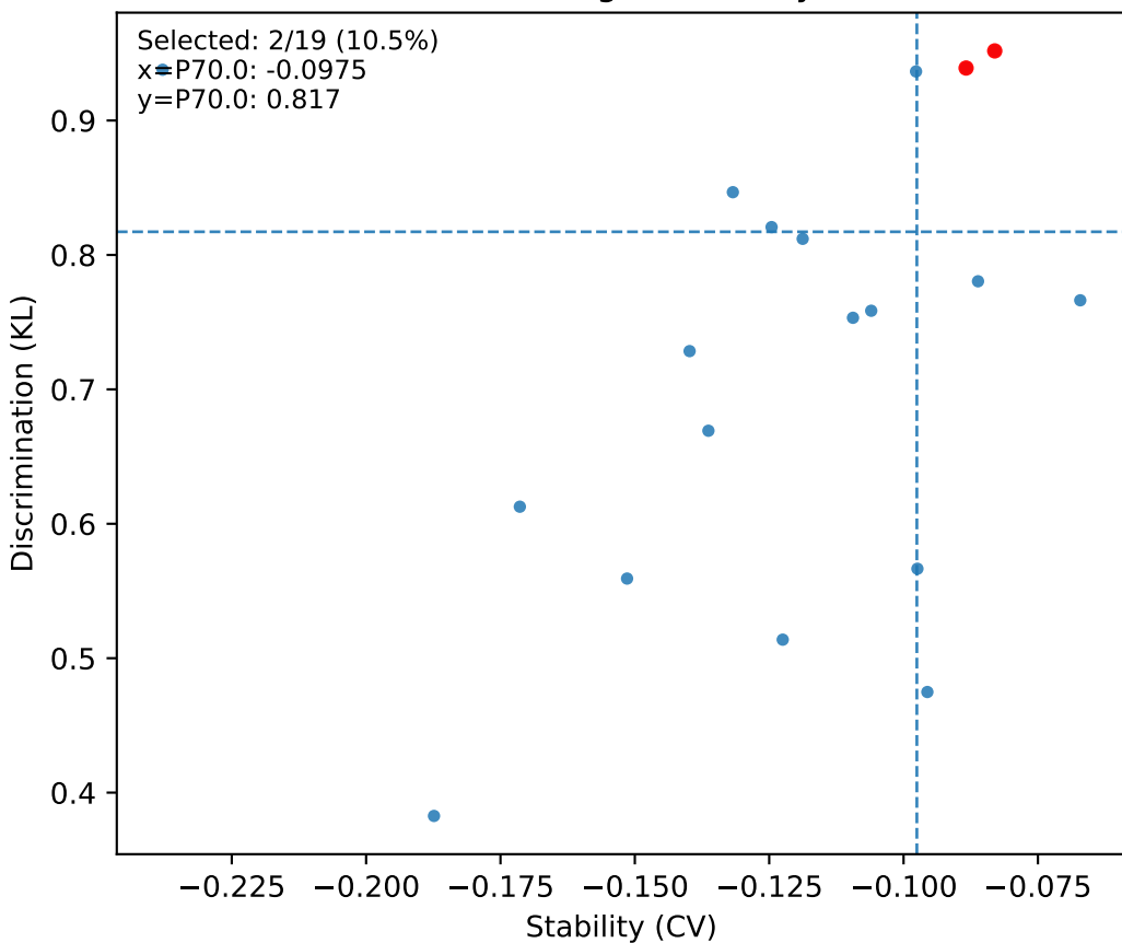
S34 Coh - Node strength: stability (-CV) vs KL
