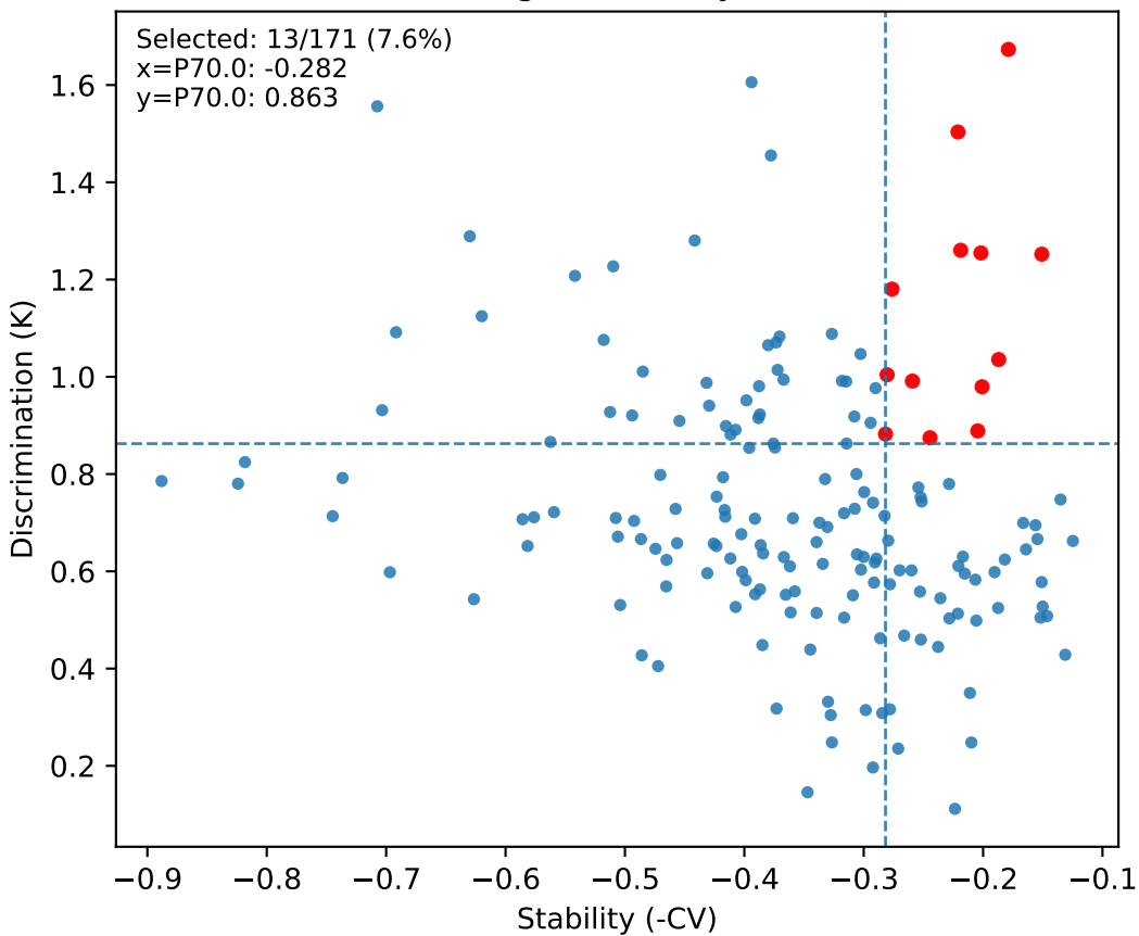
S05 CMI - Edges: stability (-CV) vs KL
