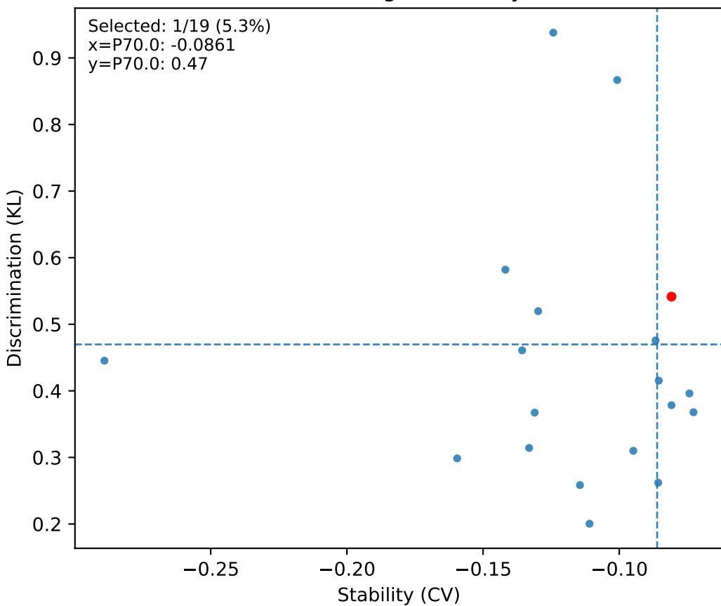
S05 Coh - Node strength: stability (-CV) vs KL
