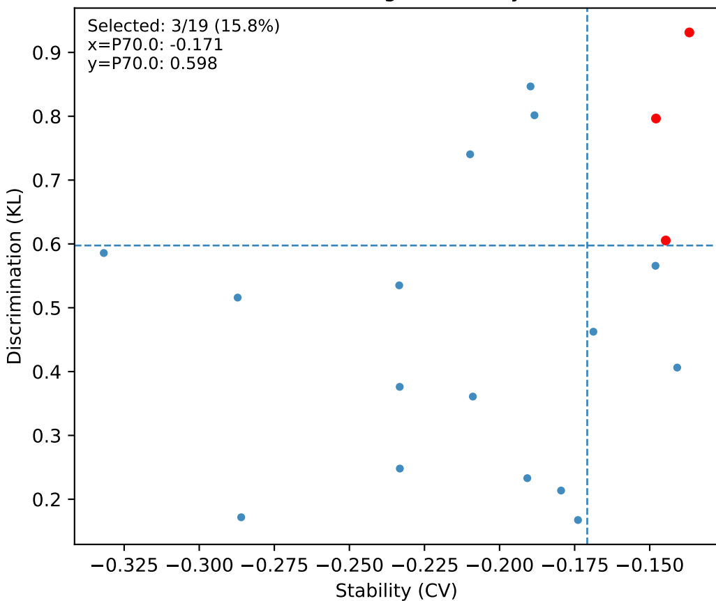
S09 MSC - Node strength: stability (-CV) vs KL
