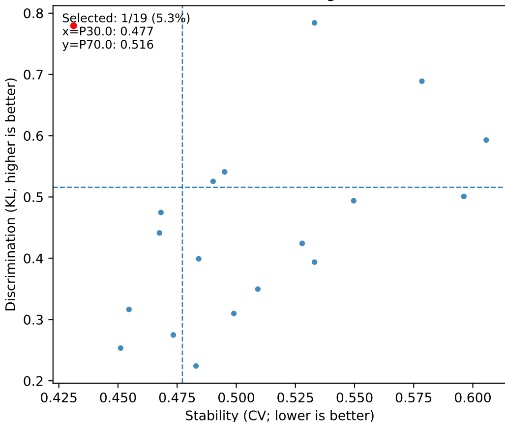
S01 imCoh — Node strength: CV vs KL
