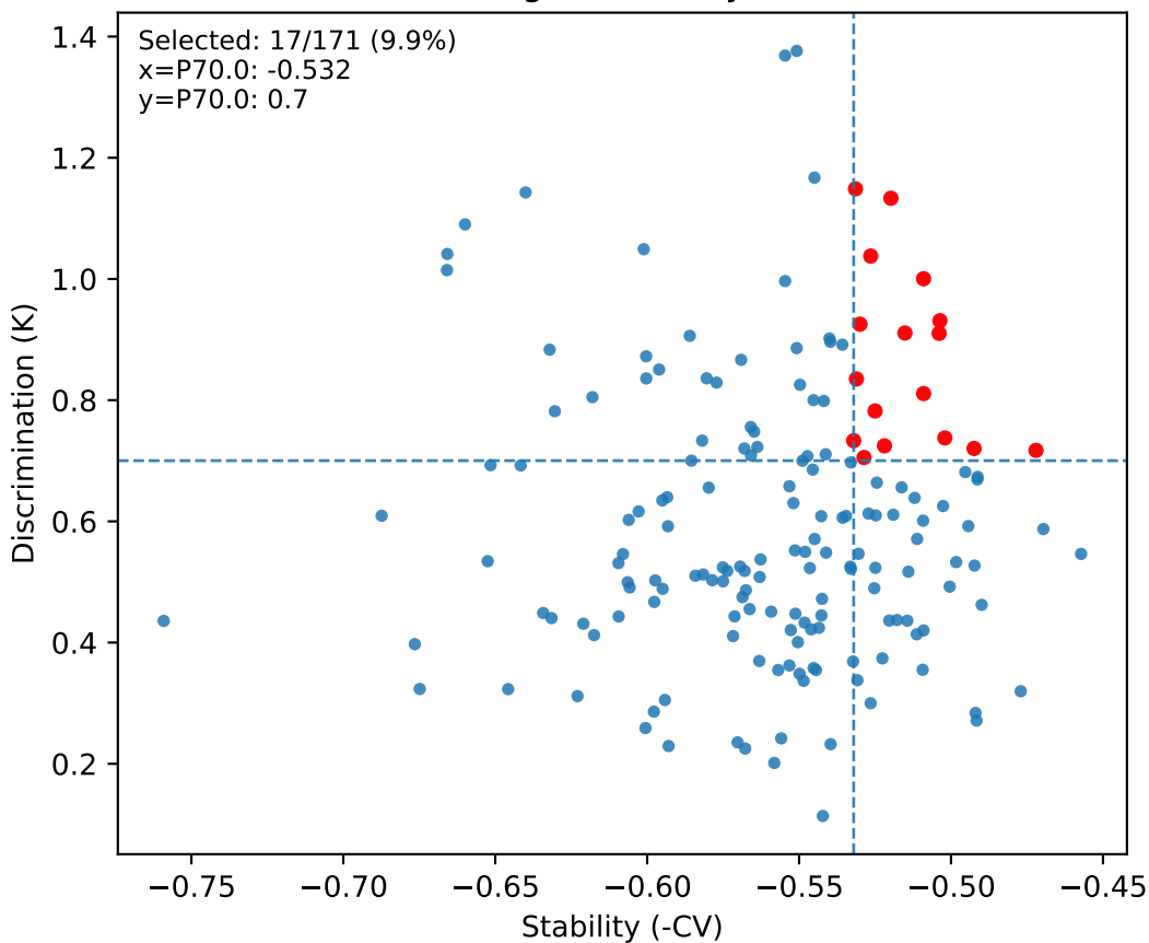
S39 CFC - Edges: stability (-CV) vs KL
