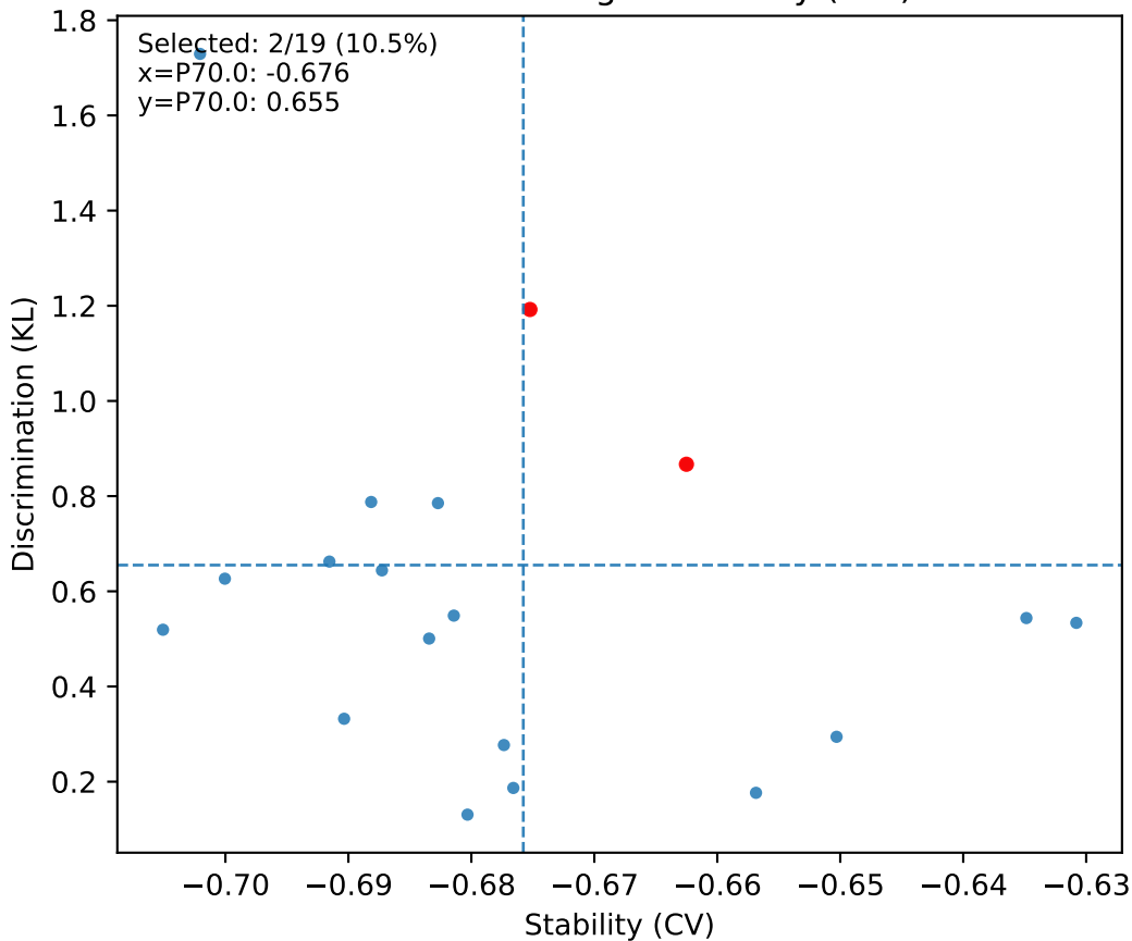
S05 CFC - Node strength: stability (-CV) vs KL
