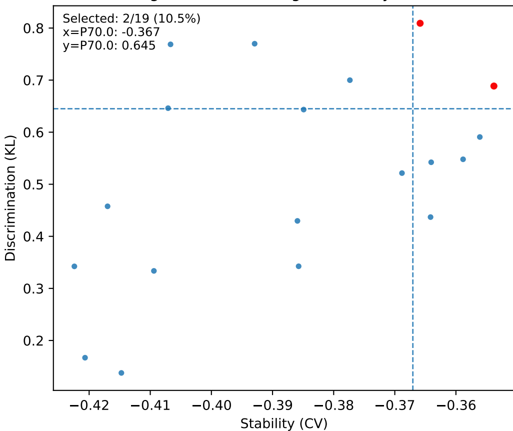
S39 ImagPLV - Node strength: stability (-CV) vs KL
