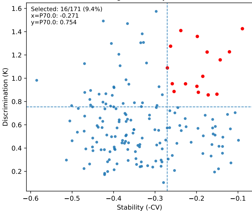
S34 CMI - Edges: stability (-CV) vs KL
