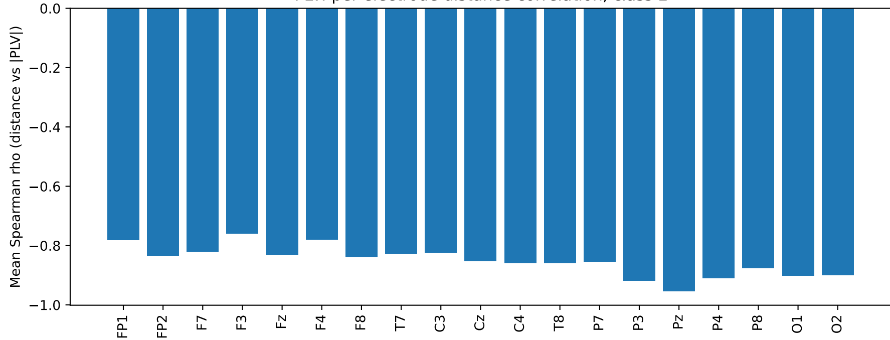
PLV: per-electrode distance correlation, class L
