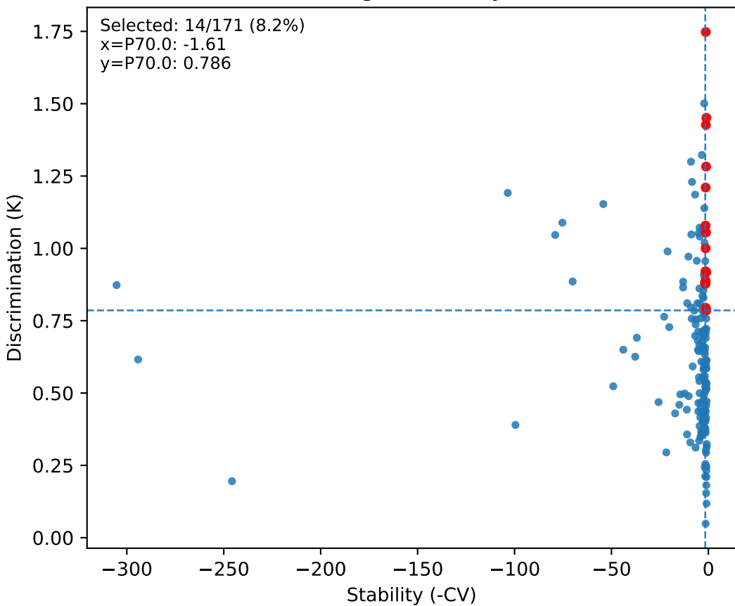
S09 imCoh - Edges: stability (-CV) vs KL
