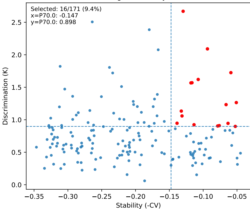
S39 MSC - Edges: stability (-CV) vs KL
