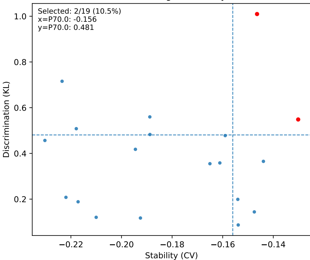
S31 MSC - Node strength: stability (-CV) vs KL
