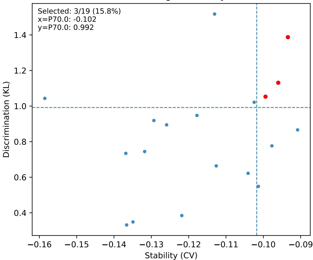
S39 MSC - Node strength: stability (-CV) vs KL
