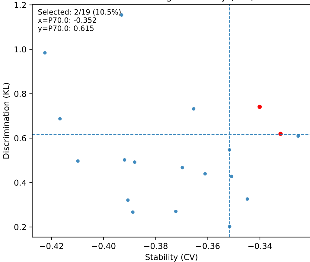
S39 wPLI - Node strength: stability (-CV) vs KL
