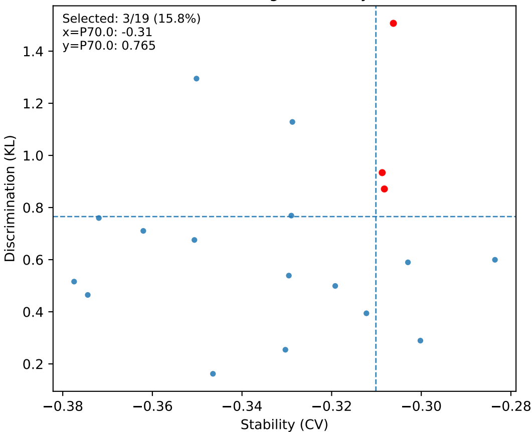
S34 PLI - Node strength: stability (-CV) vs KL
