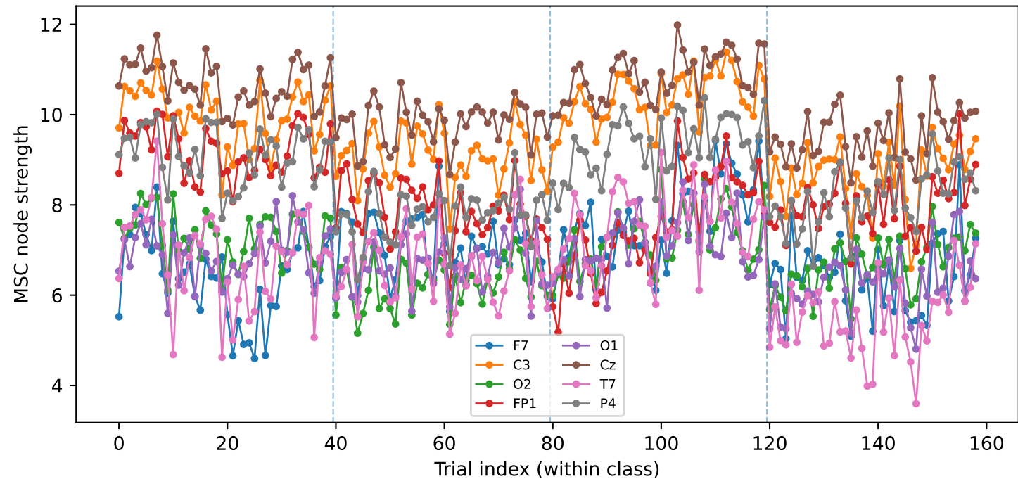
S21 MSC - NS trajectories (L)
