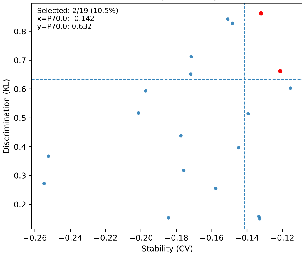
S21 CMI - Node strength: stability (-CV) vs KL
