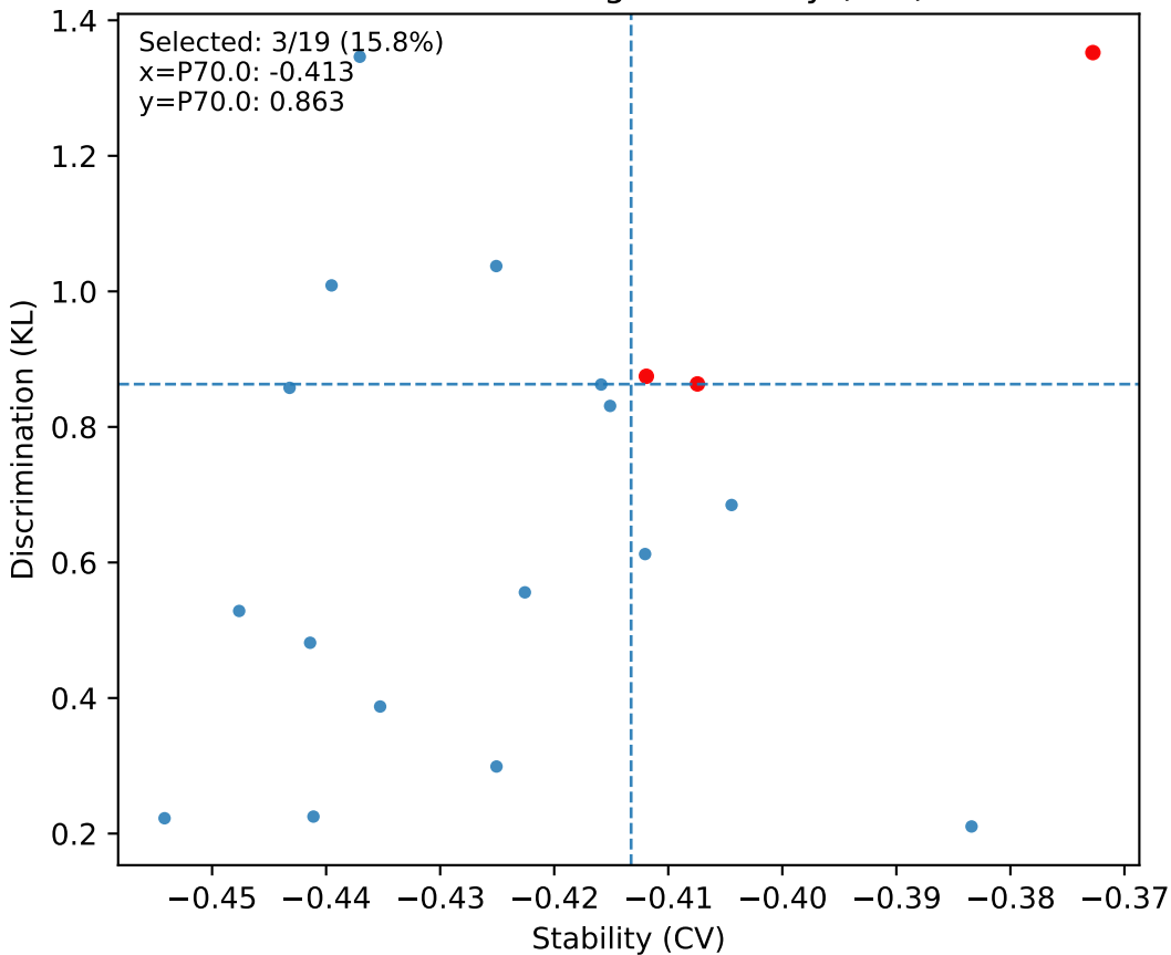
S31 CFC - Node strength: stability (-CV) vs KL
