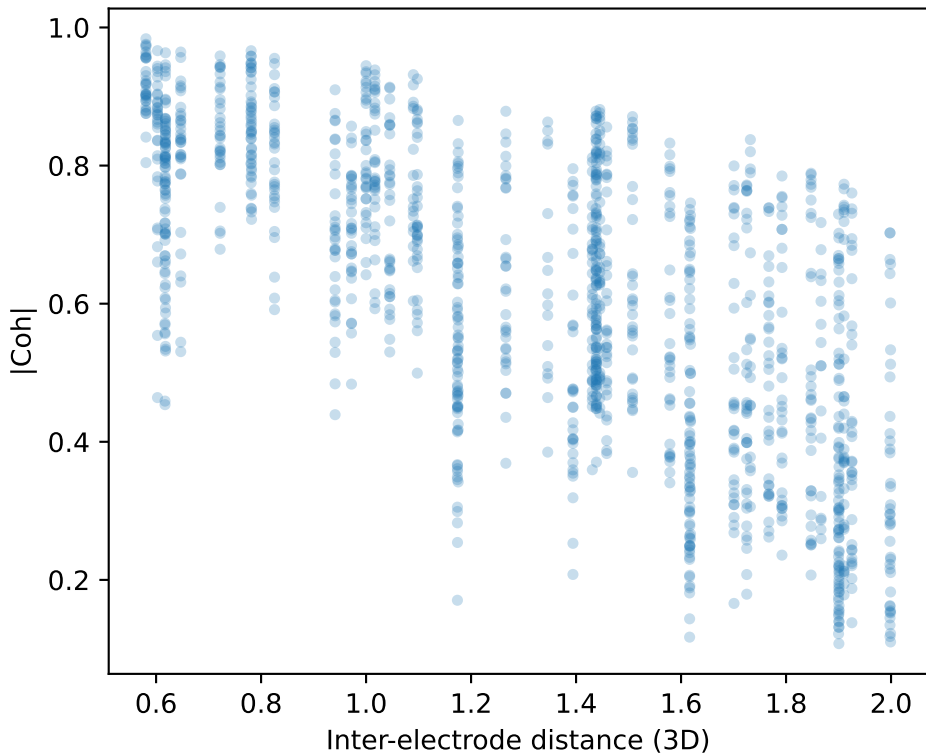
Coh vs distance, class R
