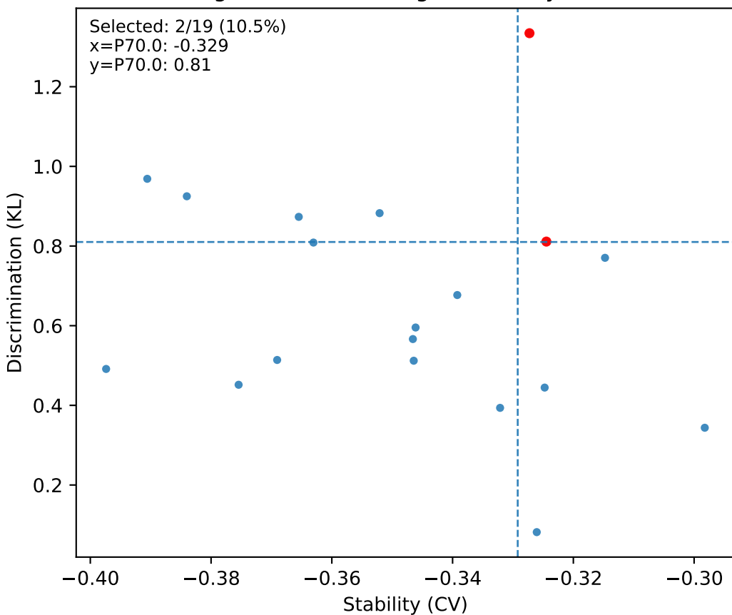
S34 ImagPLV - Node strength: stability (-CV) vs KL
