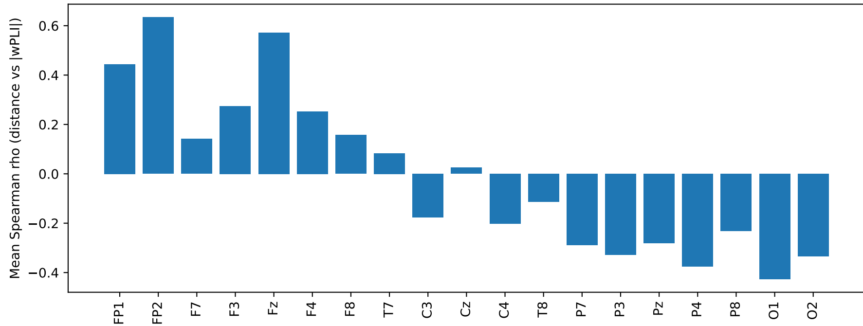
wPLI: per-electrode distance correlation, class R
