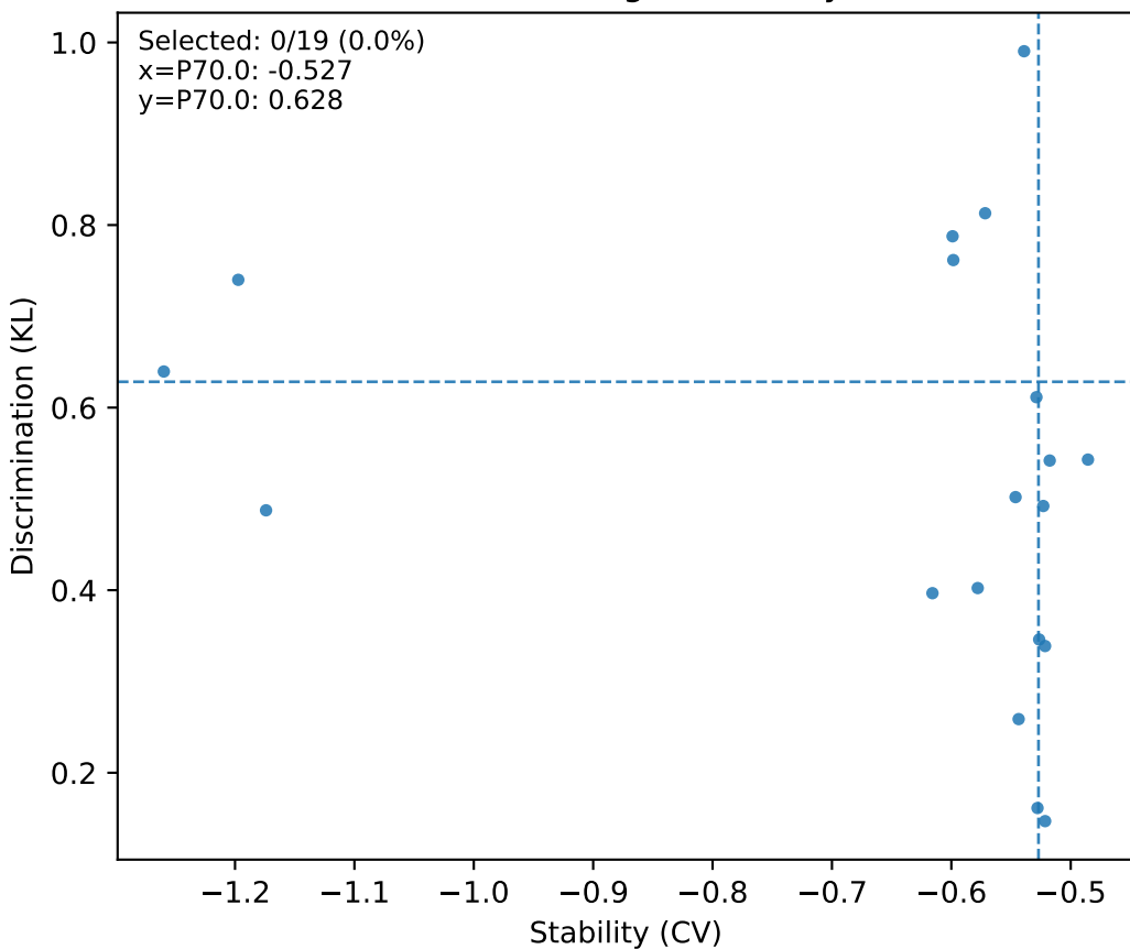
S05 imCoh - Node strength: stability (-CV) vs KL
