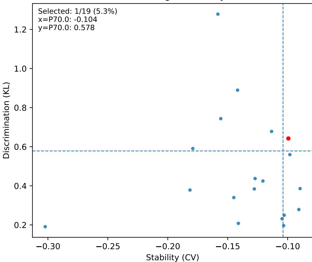
S05 PLV - Node strength: stability (-CV) vs KL
