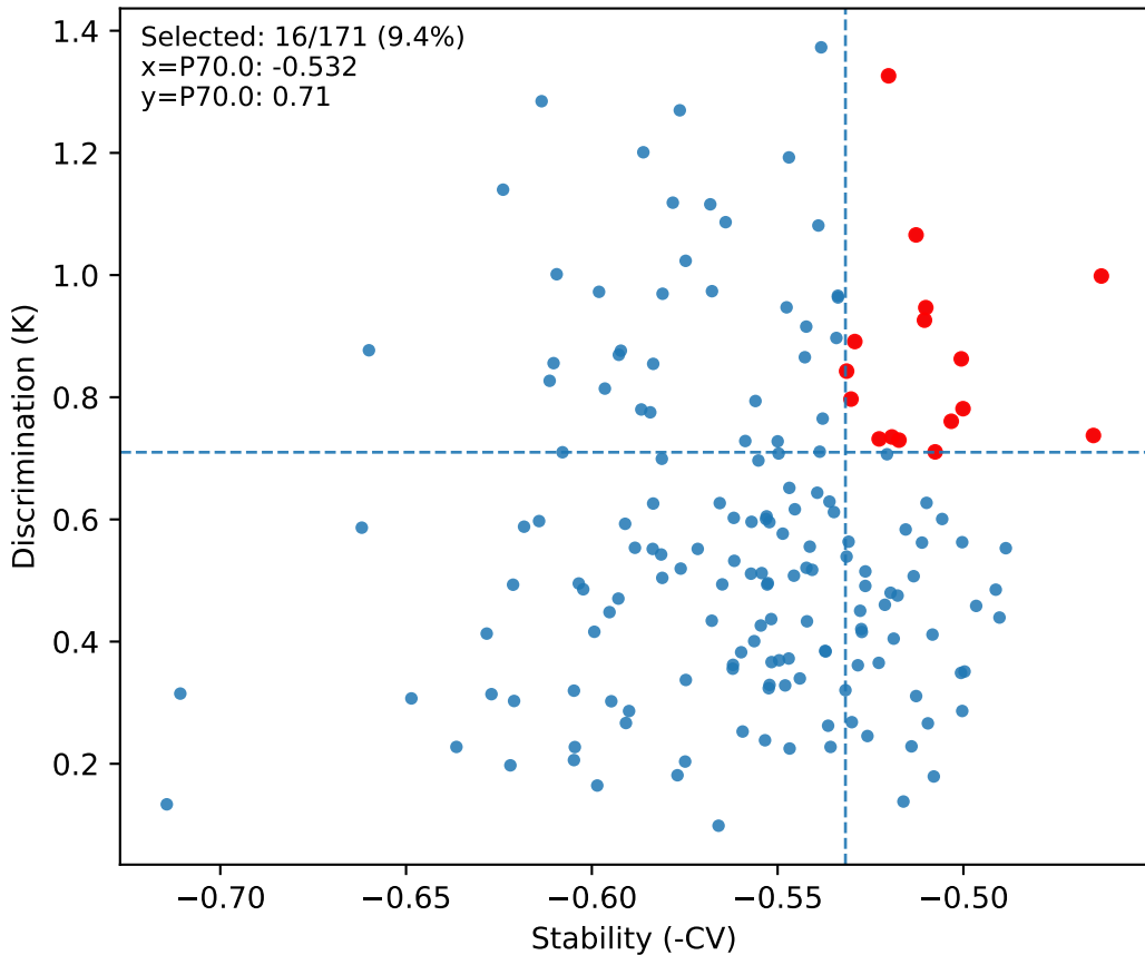
S34 CFC - Edges: stability (-CV) vs KL
