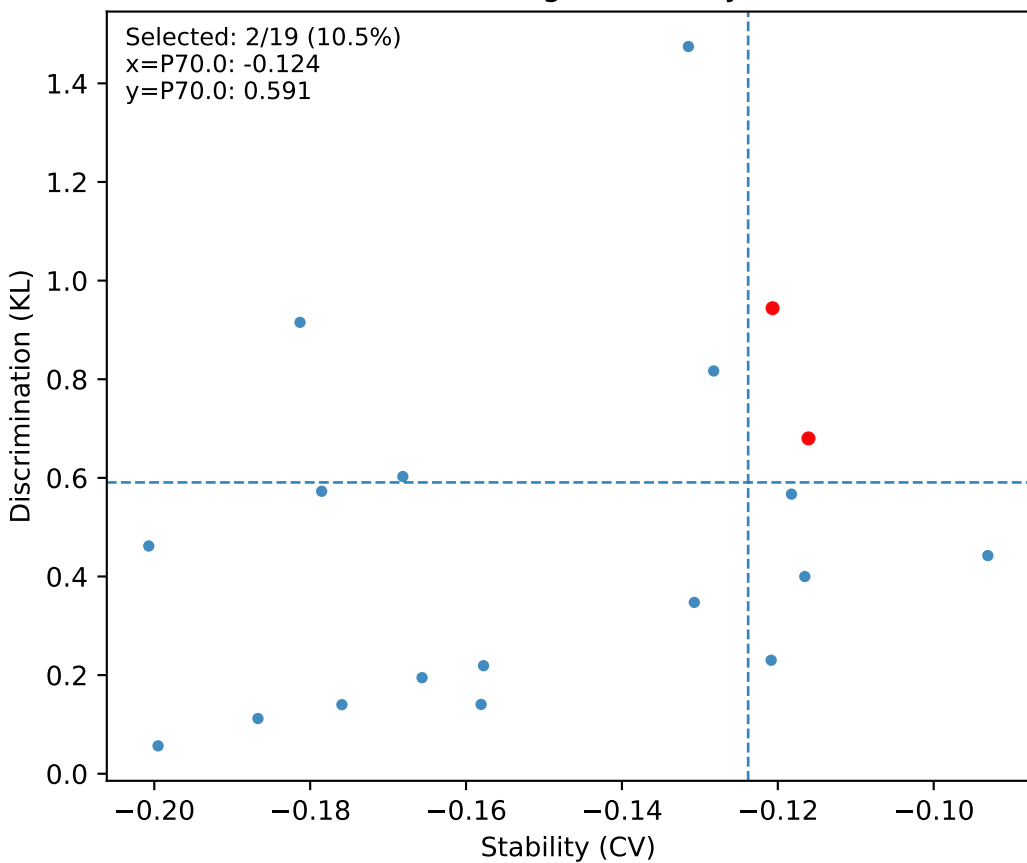
S31 PLV - Node strength: stability (-CV) vs KL
