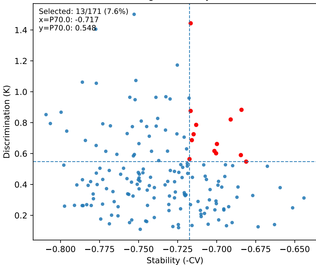
S31 wPLI - Edges: stability (-CV) vs KL
