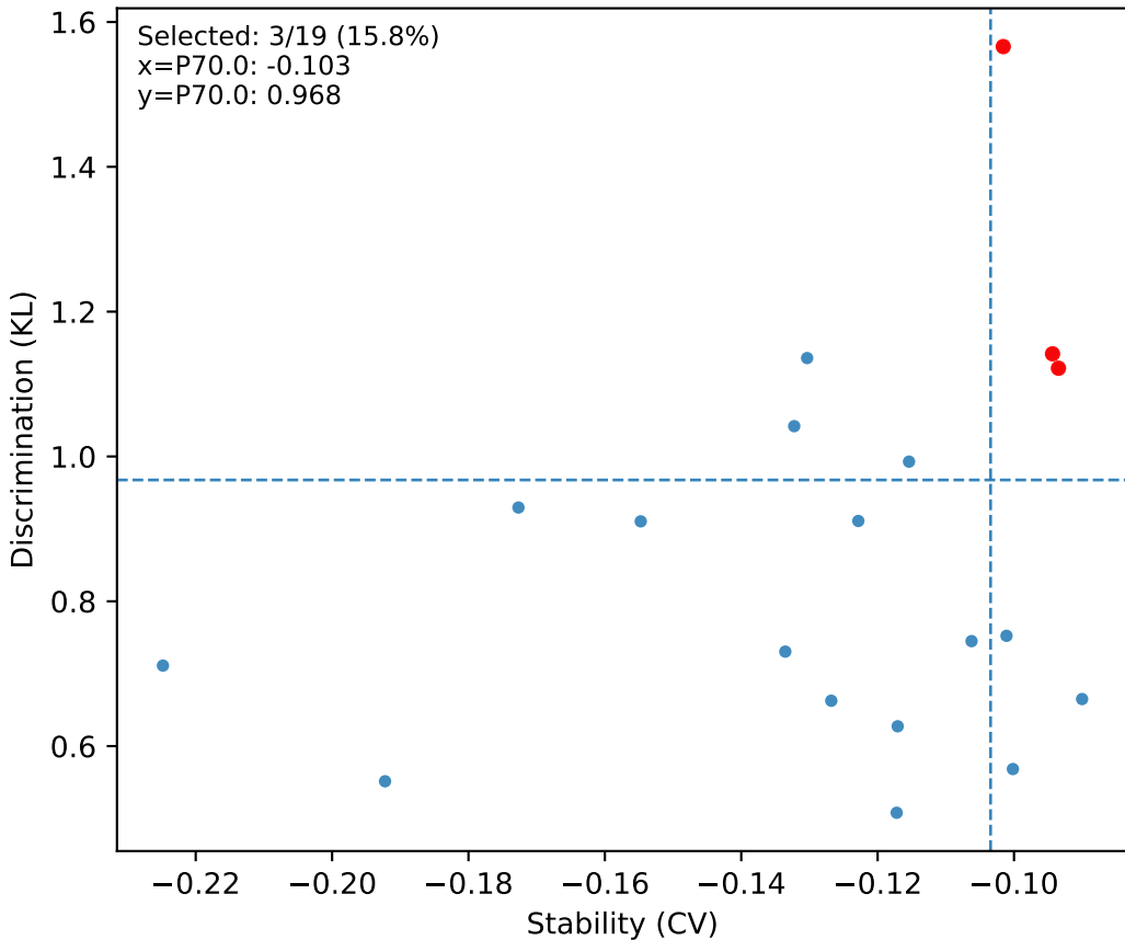
S34 MSC - Node strength: stability (-CV) vs KL
