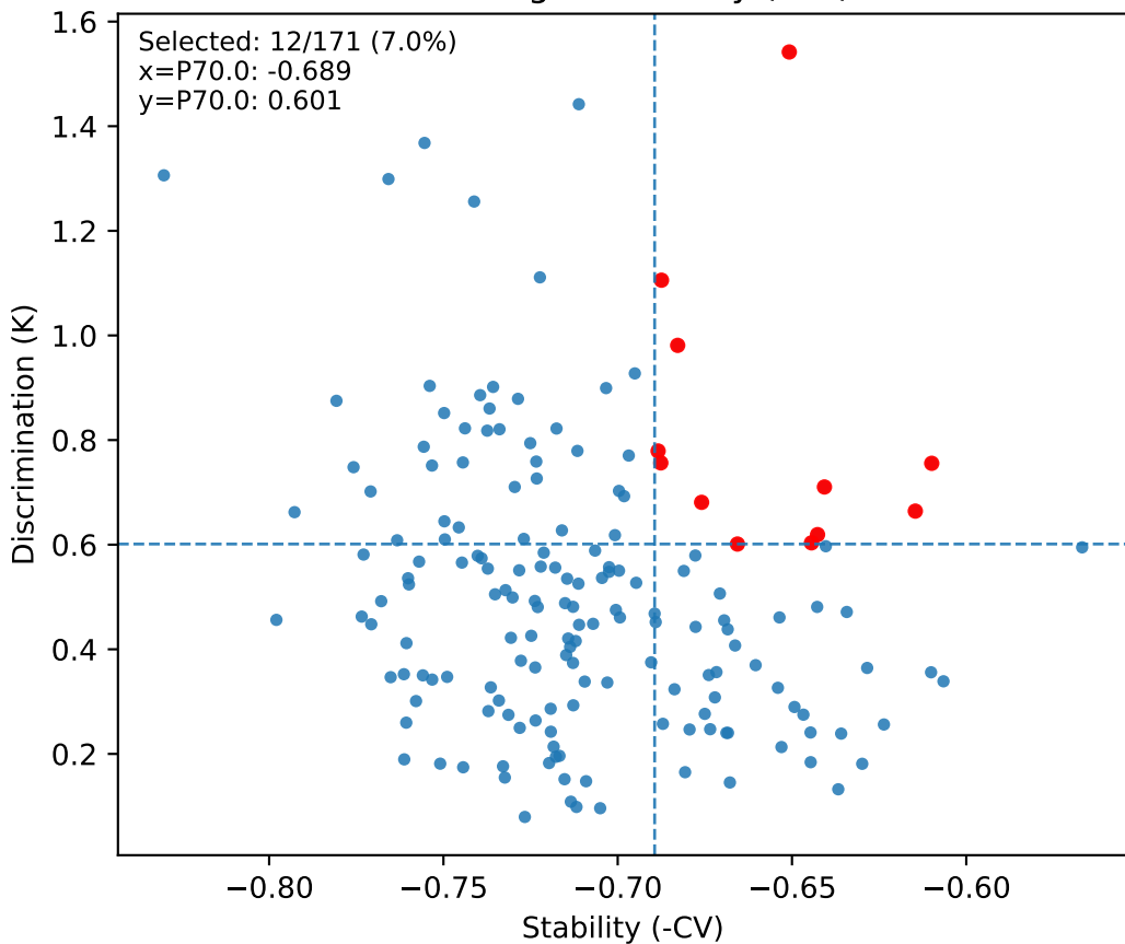
S09 wPLI - Edges: stability (-CV) vs KL
