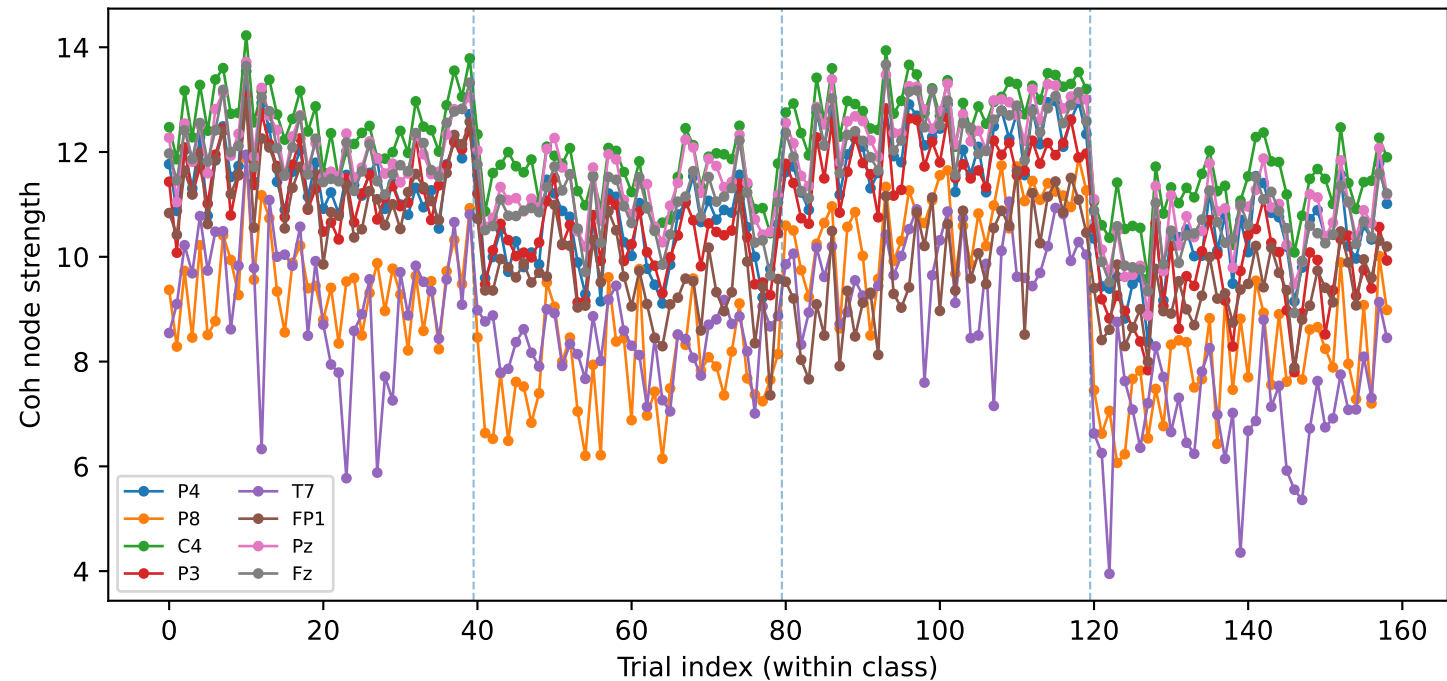
S21 Coh - NS trajectories (R)
