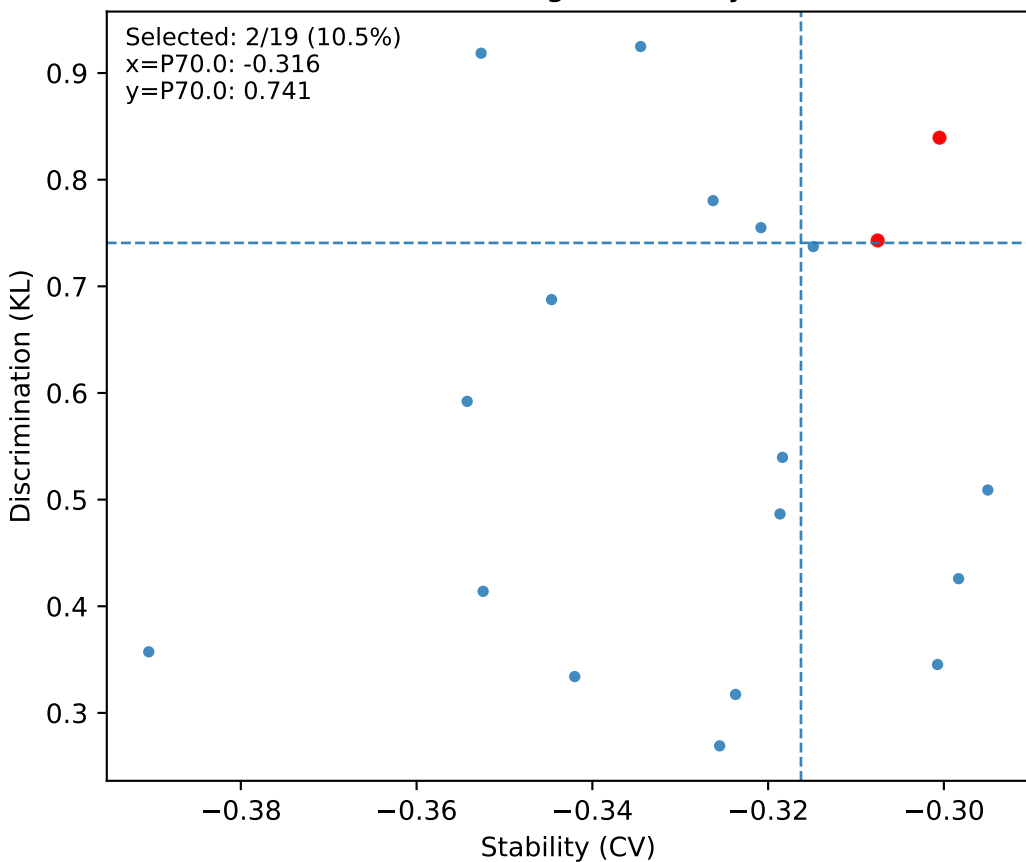
S34 CFC - Node strength: stability (-CV) vs KL
