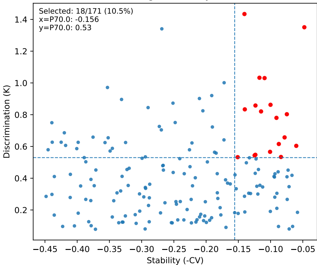
S31 MSC - Edges: stability (-CV) vs KL
