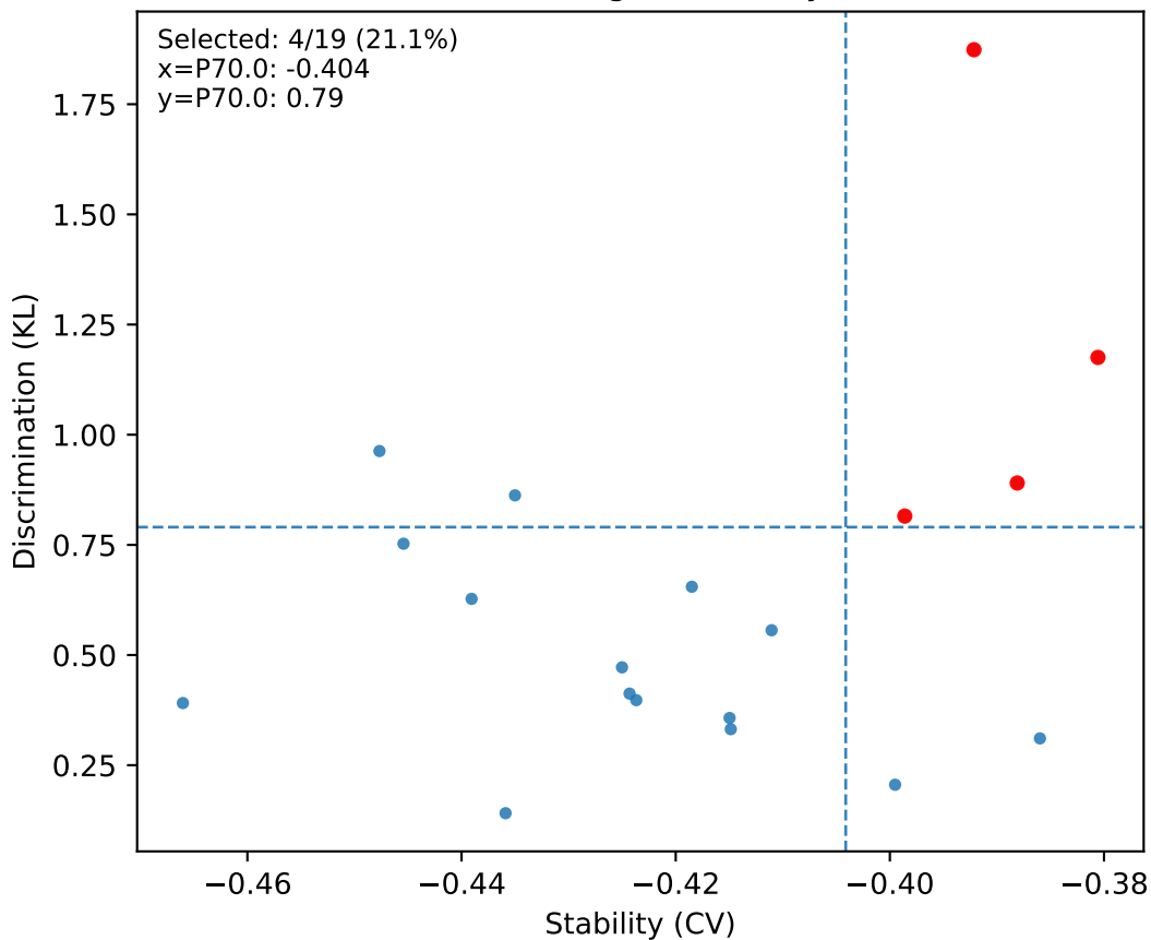
S31 PLI - Node strength: stability (-CV) vs KL
