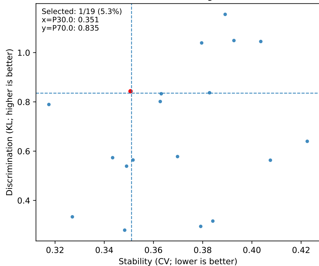
S34 imCoh — Node strength: CV vs KL
