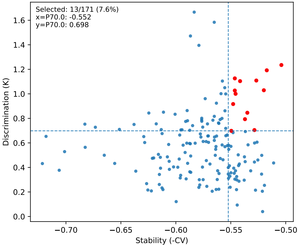
S21 CFC - Edges: stability (-CV) vs KL
