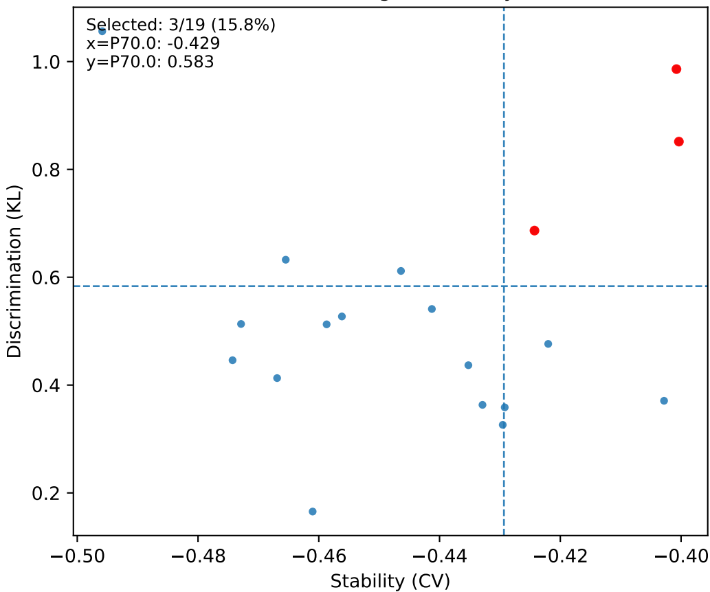
S31 wPLI - Node strength: stability (-CV) vs KL
