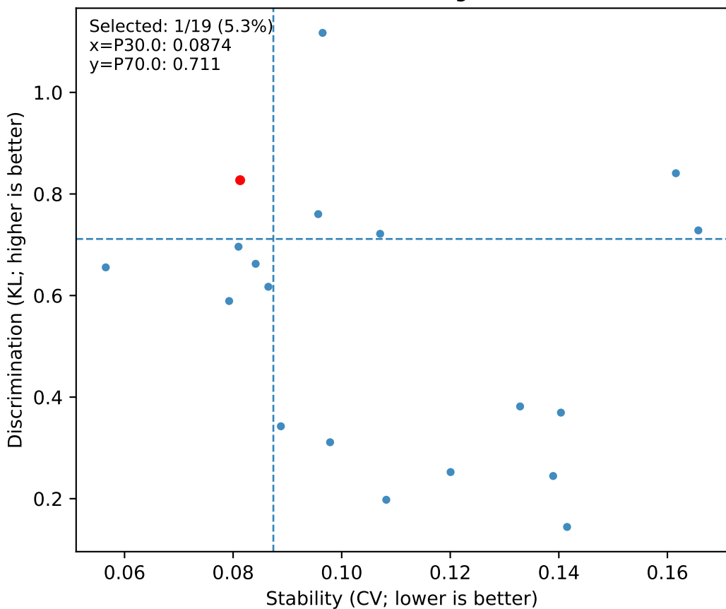
S21 Coh — Node strength: CV vs KL
