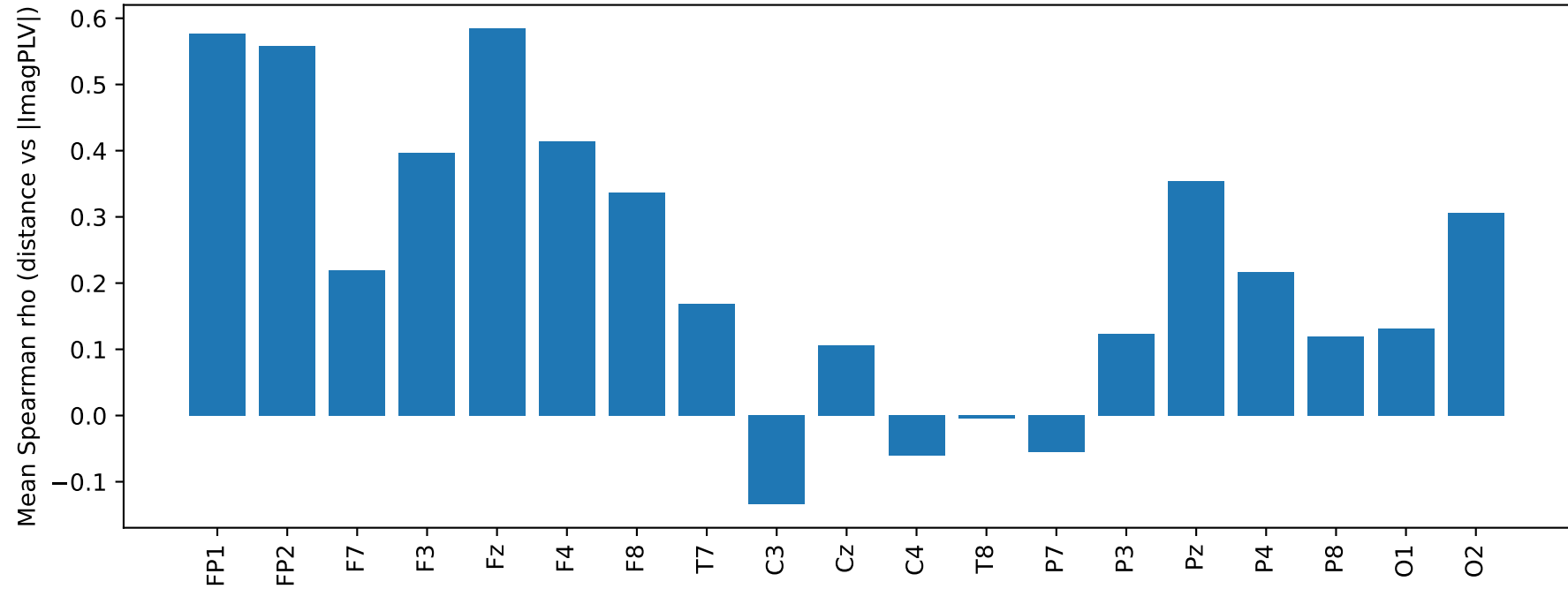
ImagPLV: per-electrode distance correlation, class R
