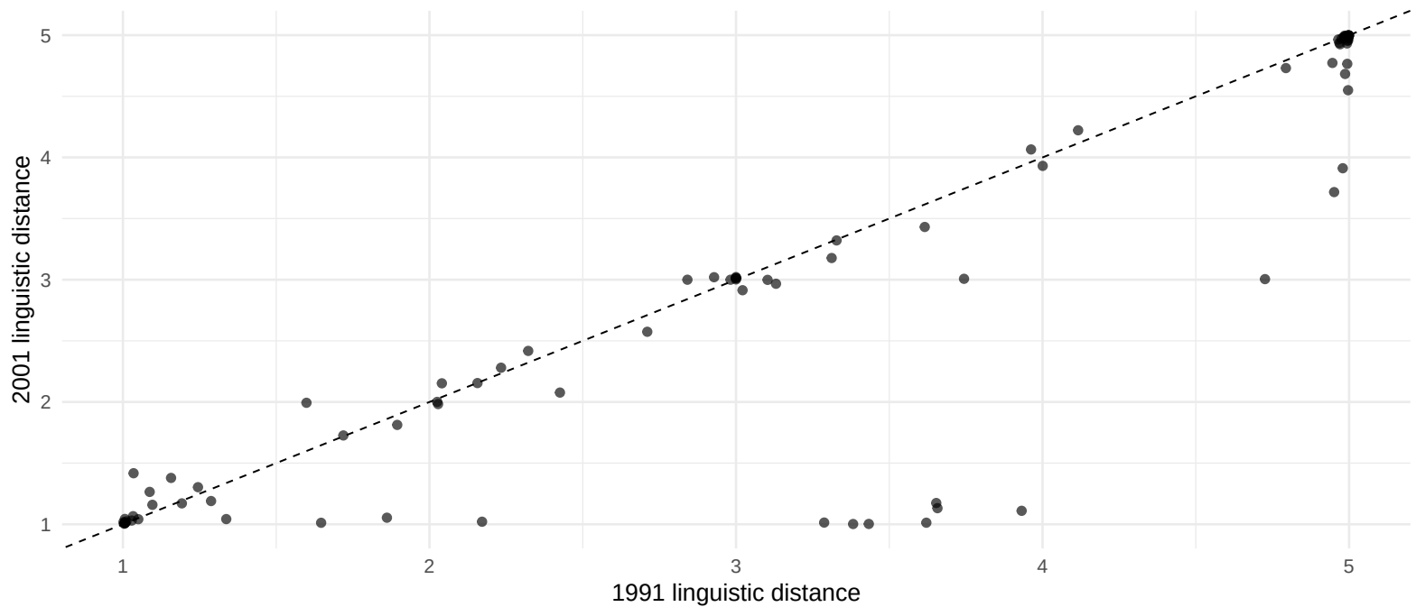
Historical persistence of linguistic distance from Hindi
