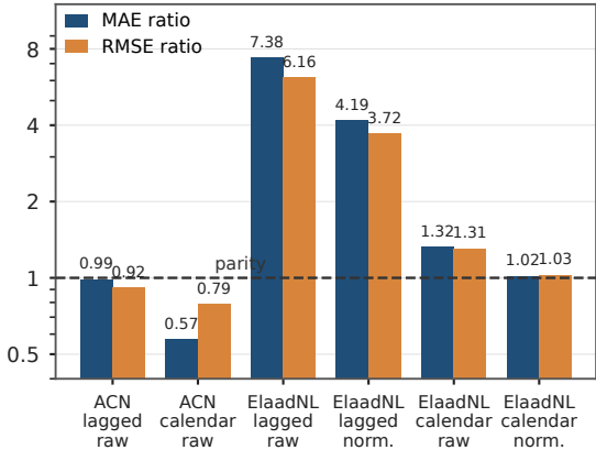
TSTR / TRTR error ratio
