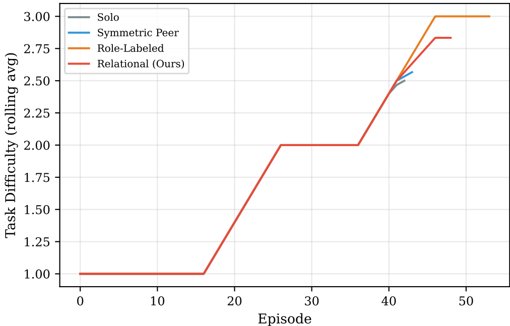
Curriculum Difficulty Progression
