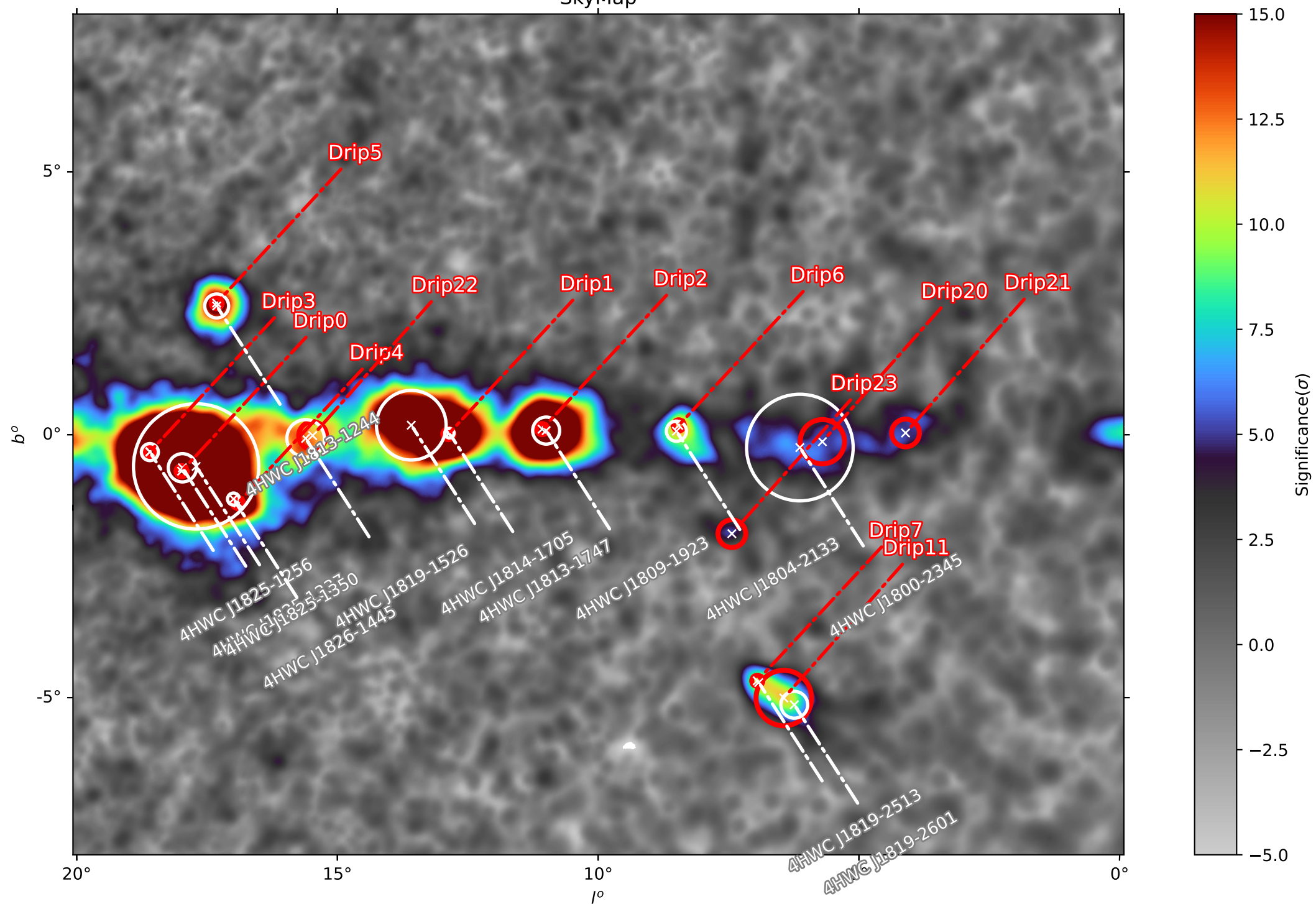
SkyMap
