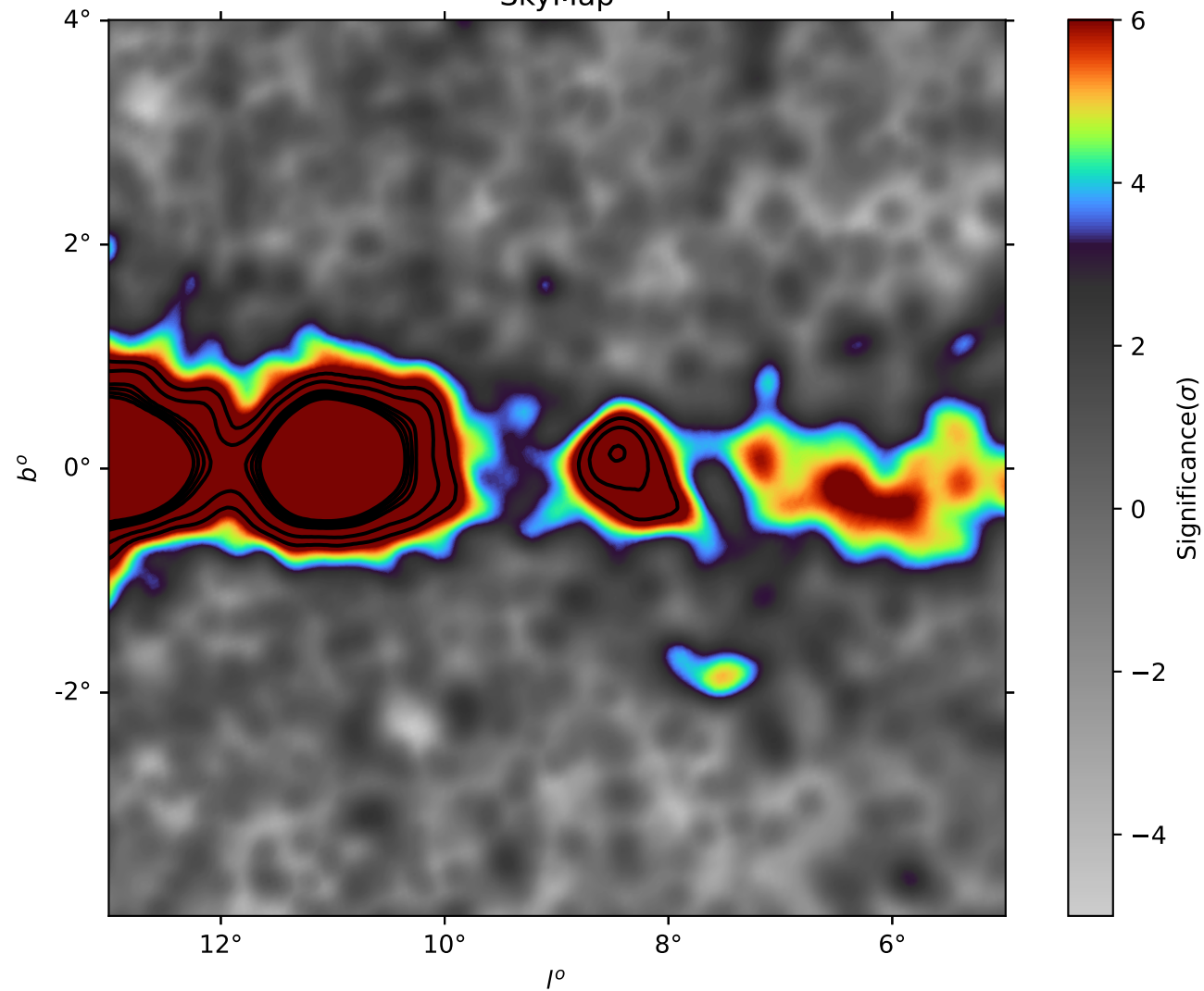
SkyMap
