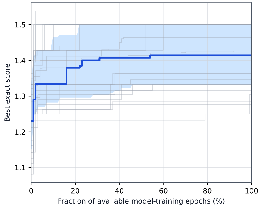
Unit-square stabbing
