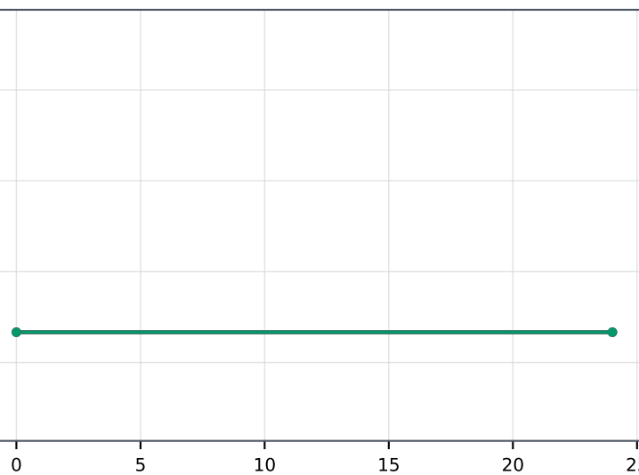
symmetry crossover hillclimb
