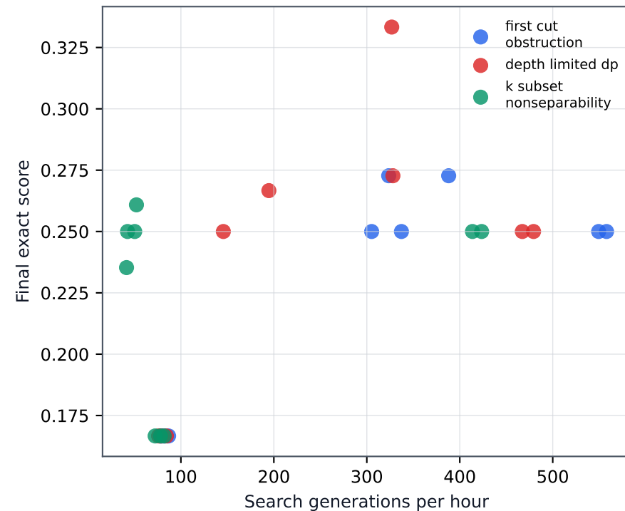
Guillotine hardness
