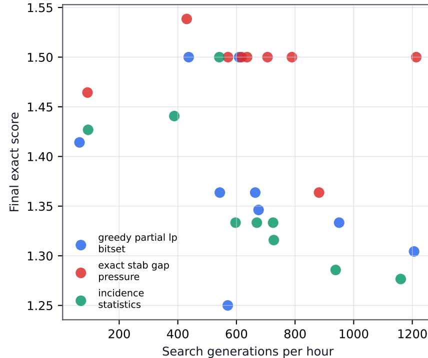
Unit-square stabbing
