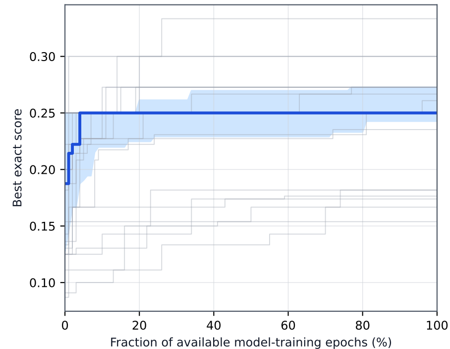
Guillotine hardness
