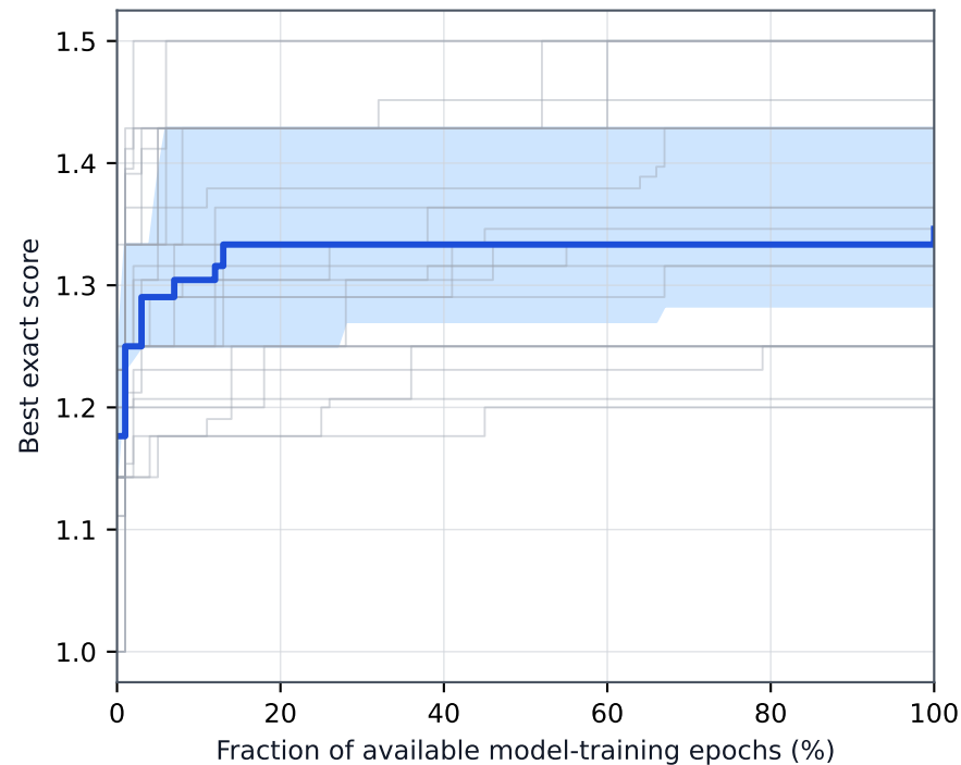
Unit-square stabbing
