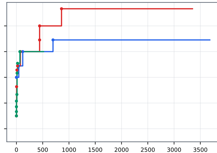
witness breaking
