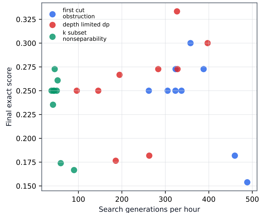
Guillotine hardness
