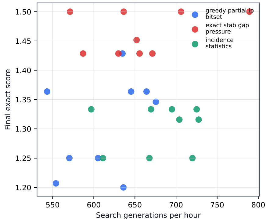
Unit-square stabbing
