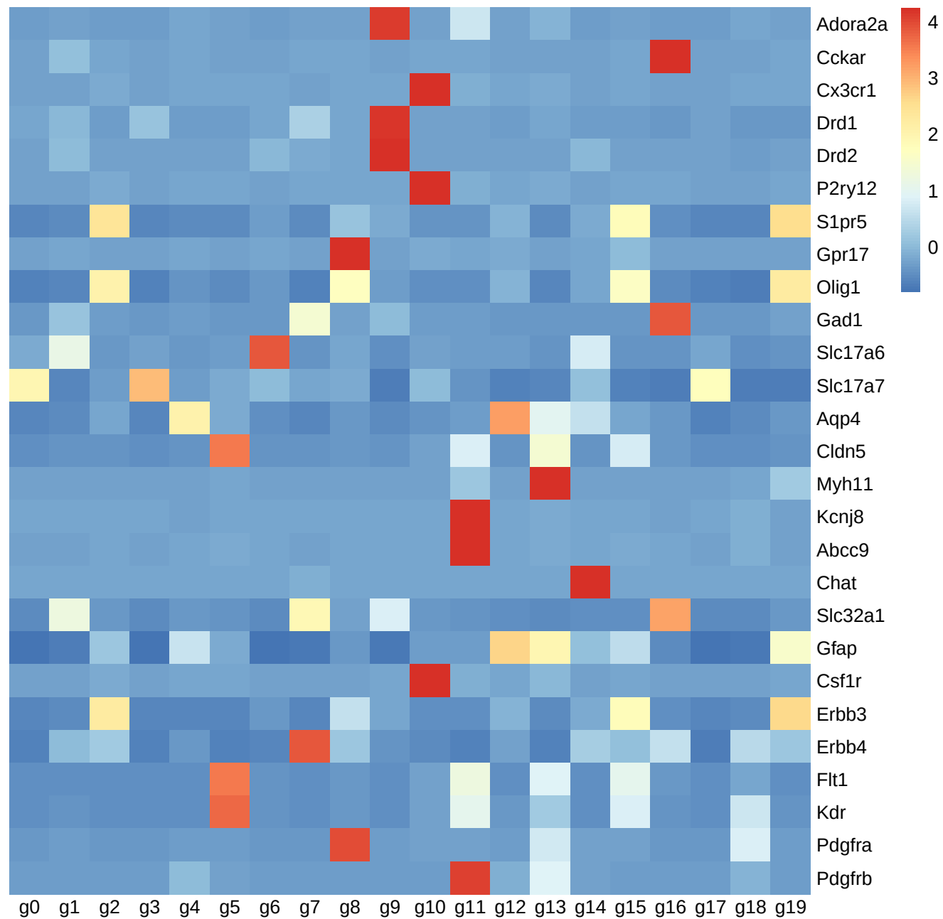
Average Marker Gene Expression Across Seurat Clusters
