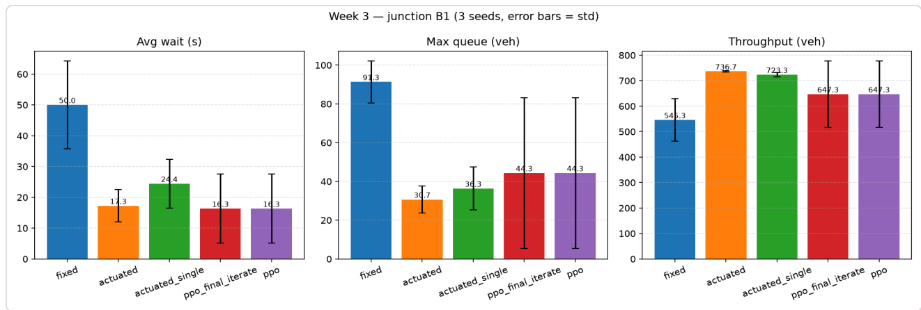
The same run measured at B1 itself, where the policy actually acts. outputs/week3_comparison_junction.png
