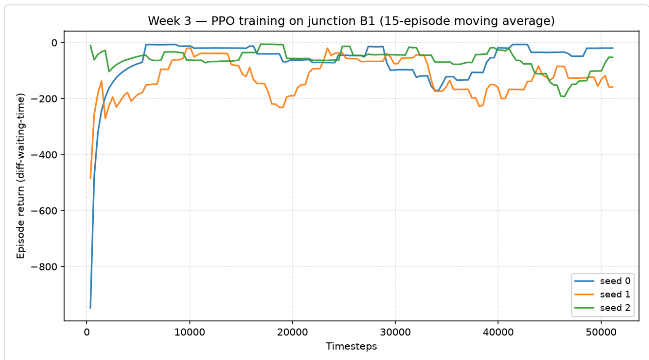
Training reward per seed. outputs/week3_reward_curves.png
