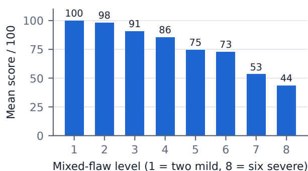
Figure 3. Mean score across the mixed-flaw gradient (Spearman \rho = -0.95 ; \rho = -0.79 between total injected severity and score over all synthetic clips). Unflawed controls score 98.4–100.
