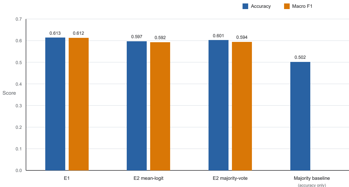
Outcome prediction on the frozen test population (n=1,503)
