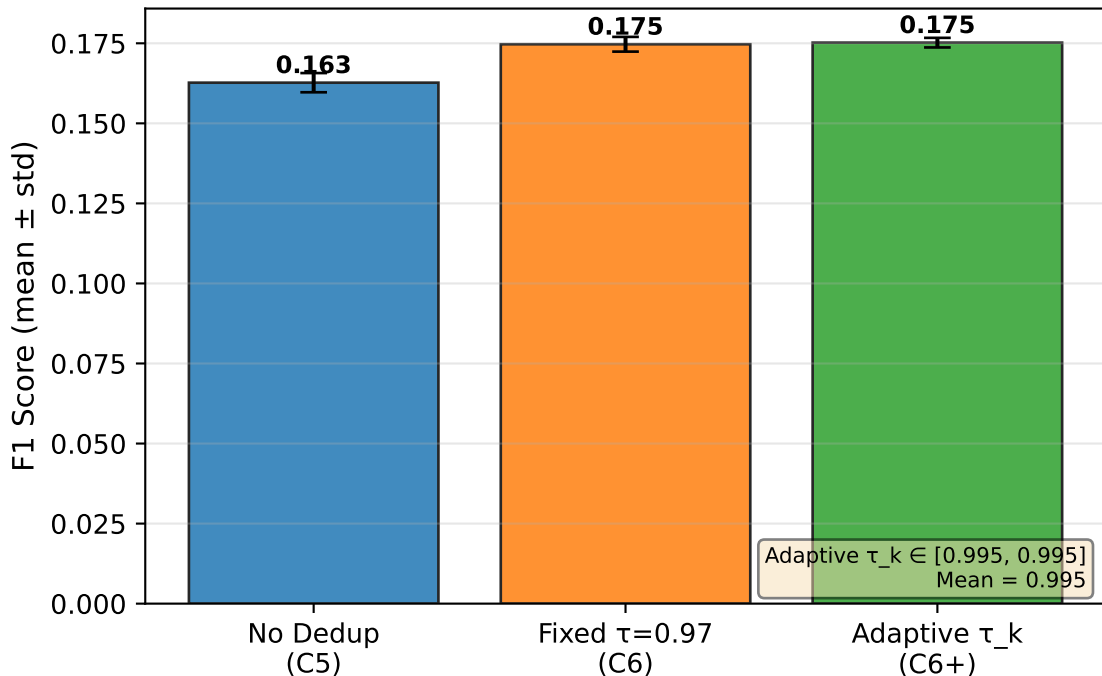
SKAB: Adaptive \tau_k vs Fixed \tau — \varepsilon=0.5 IID
