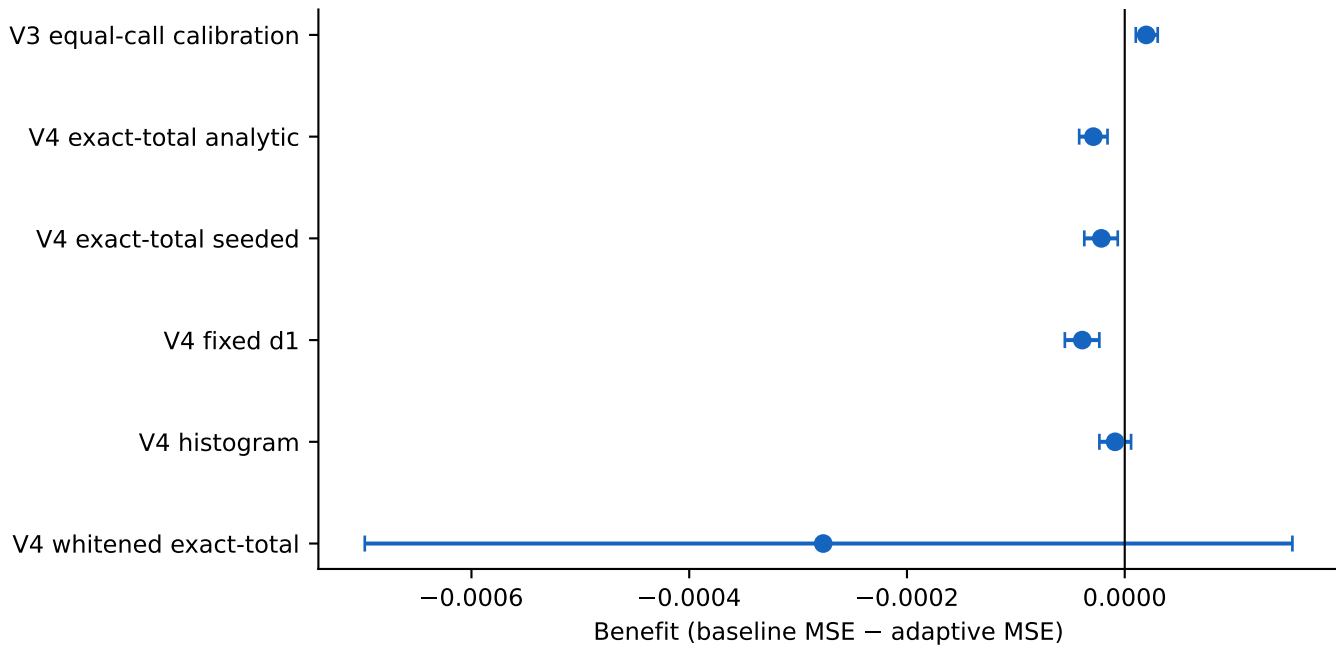
Episode-clustered 95% intervals
