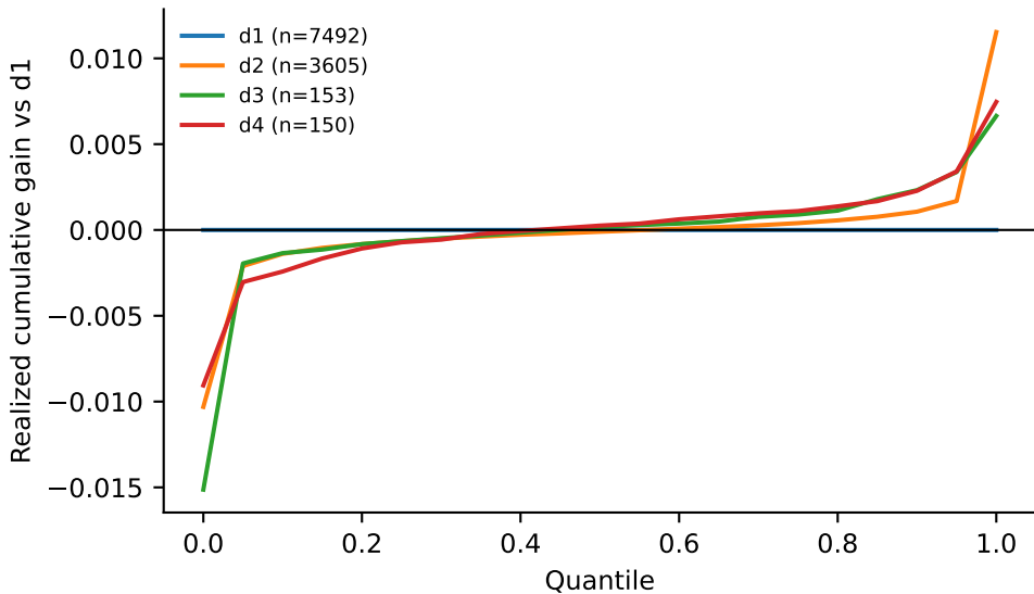
Gain quantiles by selected depth
