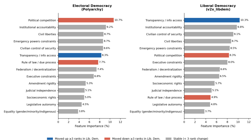
Fig. 1. CatBoost feature importances for the Polyarchy model (left) and Liberal Democracy model (right). Colour indicates rank shift: blue = moved up \geq 3 ranks; red = moved down \geq 3 ranks; grey = stable. Transparency / Information Access rises from sixth to first under Liberal Democracy; Political Competition drops from first to sixth. Judicial Independence and Legislative Autonomy remain near the bottom in both specifications.
