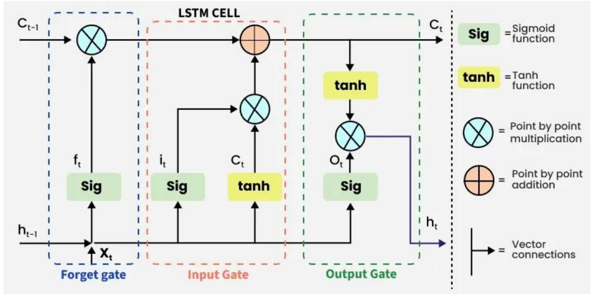
Figure 4. LSTM model architecture
