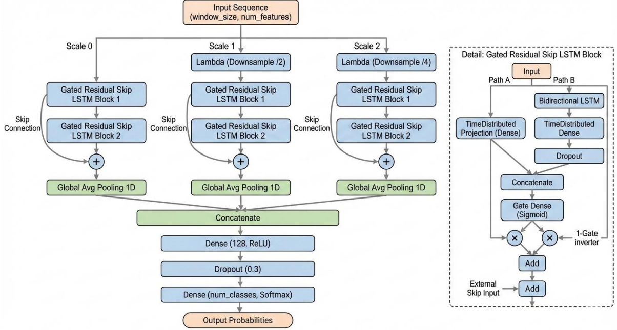
Figure 3. MS-GRS-BiLSTM model architecture
