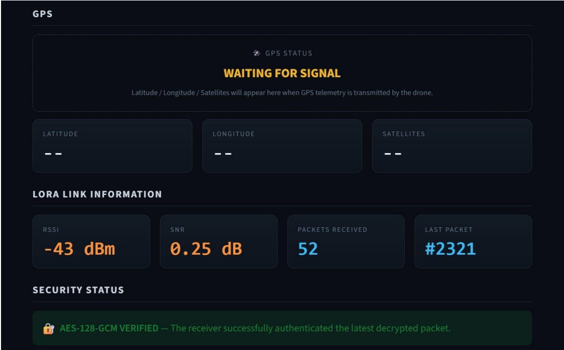
Figure 7. GPS and LoRa link information with AES-128-GCM verification status.
