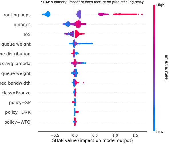
Fig. 2. SHAP summary for the XGBoost log-delay model; colour denotes feature value.
