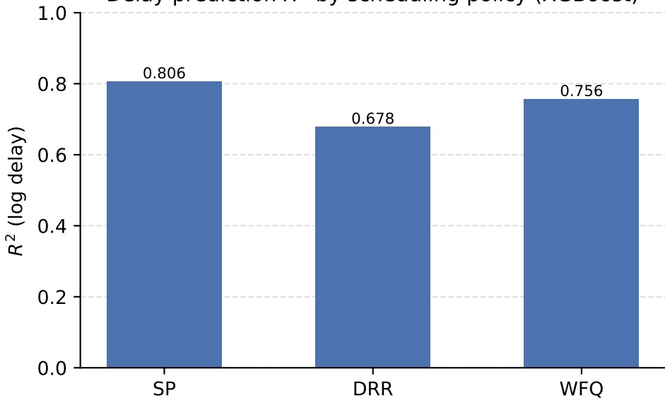
Delay prediction R^2 by scheduling policy (XGBoost)
