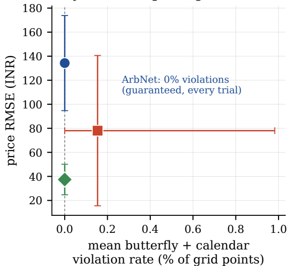
(a) Synthetic rough-Bergomi (30 trials)
